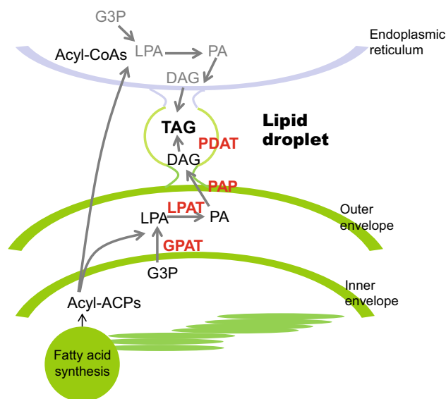
Fig. 2 One of the possible models of LD biogenesis in Chlamydomonas reinhardtii involving both plastid and ER. The TAG-synthesizing proteins present in the LD proteome are highlighted. In red are enzymes; in black are lipid substrates. This model is partly based on that of (Goodson et al. 2011; Nguyen et al. 2011). ACP acyl carrier protein, CoA coenzyme A, DAG diacylglycerol, G3P glycerol-3-phosphate, GPAT glycerol-3-phosphate acyltransferase, LPA lysophosphatidic acid, LPAT lysophosphatidic acid acyltransferase, PA phosphatidic acid, PAP phosphatidic acid phosphatase, PDAT phospholipid:diacylglycerol acyltransferase, TAG triacylglycerol
