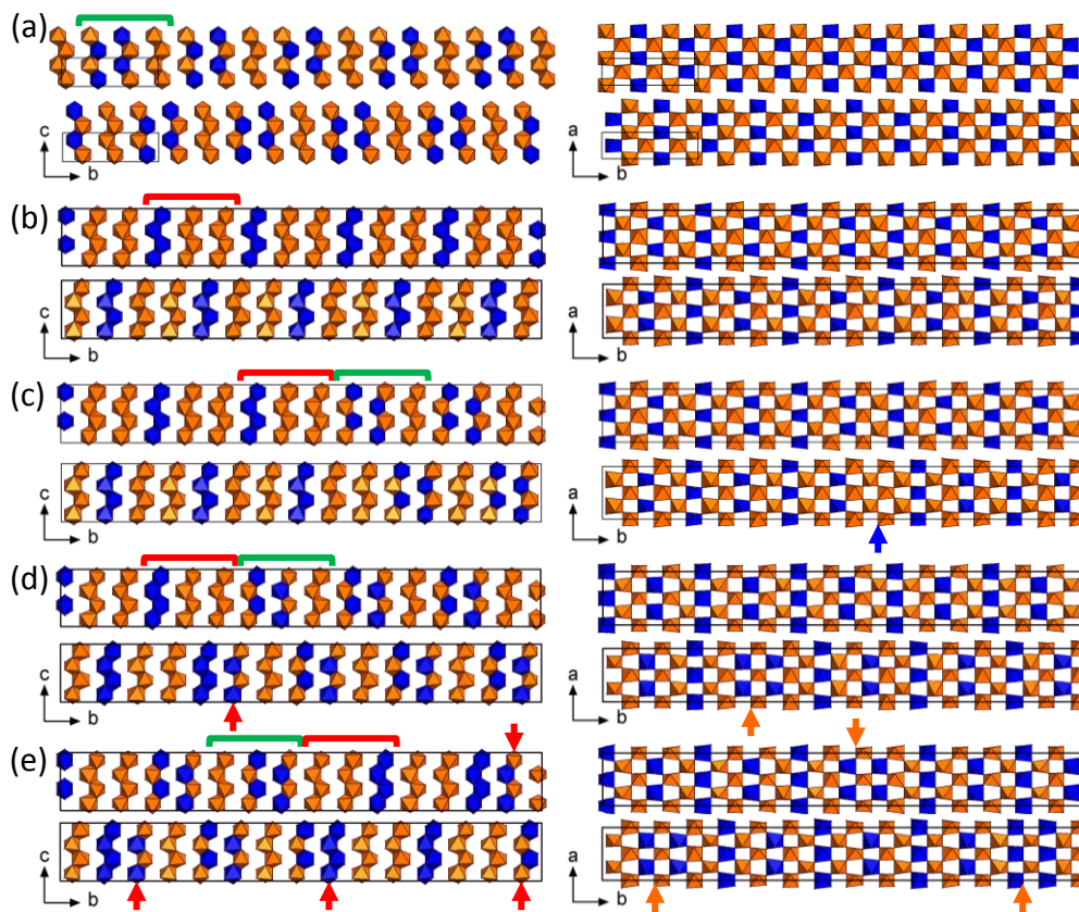
Figure 5. Representation of cation ordering in the bc (left panel) and ab (right panel) planes in Fe 2 WO 6 samples considering different structural models. (a) 2x5x2 supercell in the Pbcn space group (b-e) 3D 2x15x2 supercells generated from the Pbcn (0 \beta 0)000 superspace group, commensurate case (b) \beta = 2/3 , incommensurate cases (c) \beta = 0.6687(4) , (d) \beta = 0.670(3) and (e) \beta = 0.697(15) . Color scheme: WO 6 octahedra, blue; FeO 6 octahedra, orange.
