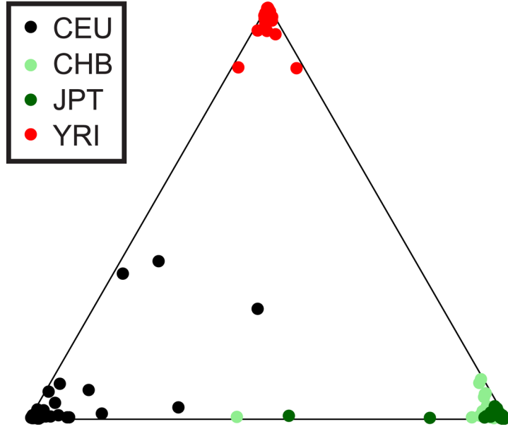
Figure 7. Population clustering from CNV genotypes A triangle plot showing the clustering of 210 unrelated HapMap individuals assuming three ancestral populations ( k=3 ). The proximity of an individual to each apex of the triangle indicates the proportion of that genome that is estimated to have ancestry in each of the three inferred ancestral populations. The clustering together of most individuals from the same population near a common apex indicates the clear discrimination between populations obtained through this analysis. The clustering was qualitatively similar to that obtained previously with a similar number of biallelic Alu insertion polymorphisms on different African, European and Asian population samples 60.
