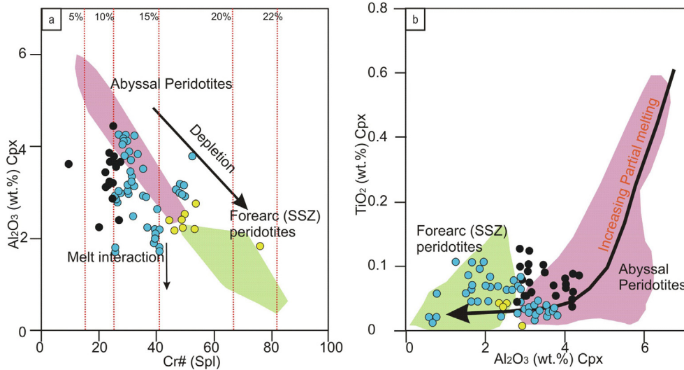
Fig. 17. Variation diagrams of a) Al_2O_3 (wt.%) clinopyroxene versus Cr\# [100Cr/(Cr + Al)] of coexisting spinel. b) TiO_2 (wt.%) versus Al_2O_3 wt.% contents in clinopyroxene of the Spontang peridotites.
