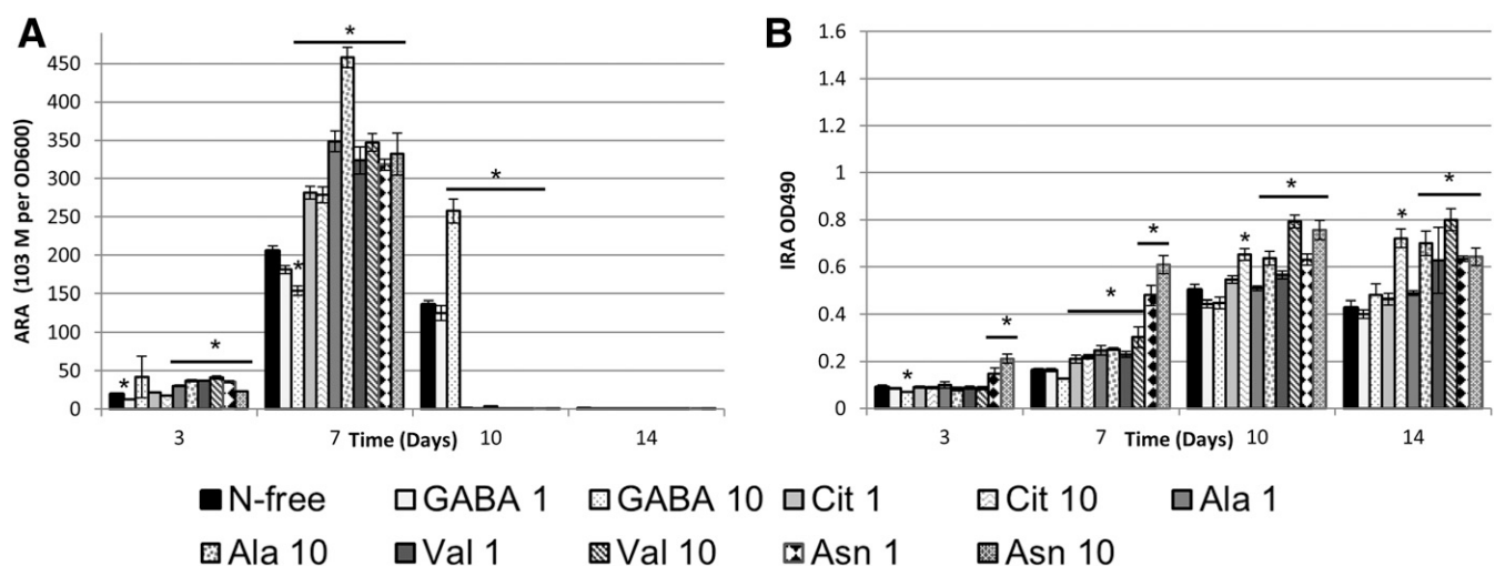
Fig. 4. A , Effects of \gamma -amino-n-butyric acid (GABA), citrulline (Cit), alanine (Ala), valine (Val), and asparagine (Asn) on Frankia ACN14a nitrogen fixation and B , respiration rates. Amino acids were tested at two different concentrations, 1 and 10 mM, under N-fixing conditions (N-free media). Asterisks (*) indicates significant difference observed compared with the control (N-free) for the same time ( P value < 0.05)
