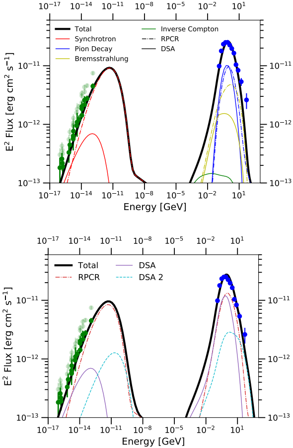
Fig. 12. Same as Fig. 11, but the multiwavelength model has multiple contributions. Upper panel: DSA scenario (solid lines) and RPCR scenario (dot-dashed lines). The total contribution from the two scenarios is shown by the solid black line. Lower panel: same as the upper panel, but with contribution from the intercloud region (DSA 2).
