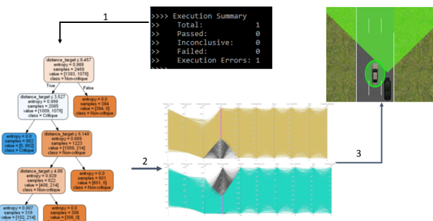
Figure 2. Investigation of the causes of the crash: 1) decision tree, 2) parallel coordinates, 3) visualization of the field of view.
