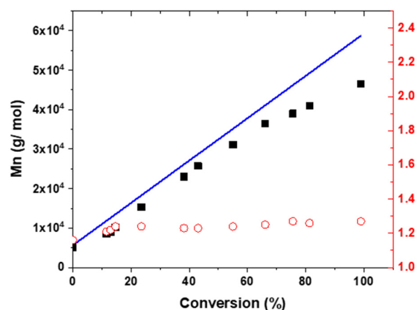
Figure 2. Evolution of number-average molar mass ( M_n , black squares) and dispersity ( \bar{D} , red open circles) with conversion for the RAFT dispersion polymerization of HFBMA at 10% w/w solids in ethanol at 70 °C using a PDMA 39 macro-CTA with macro-CTA/AIBN molar ratio of 5/1. The targeted diblock composition was PDMA 39 -PHFBMA 200 .
