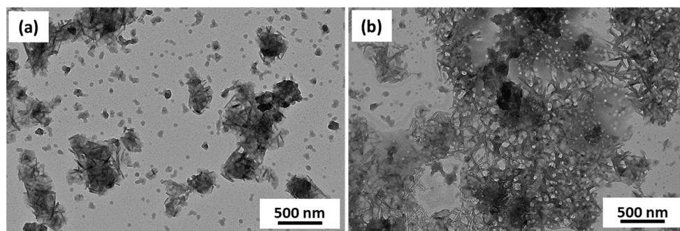
Figure 6. TEM images obtained for PDMA 58 -PBzMA 198 -PHCFDDMA x prepared at 10% w/w with (a) x = 19 (b) x = 50 .
