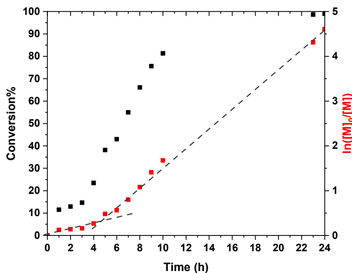
Figure 1. Kinetic data (Conversion %: Black squares, Semi-log: Red squares) obtained for the RAFT dispersion polymerization of HFBMA at 10% w/w solids in ethanol at 70 °C using a PDMA 39 macro-CTA at a macro-CTA/AIBN molar ratio of 5/1. The targeted diblock composition was PDMA 39 –PHFBMA 200 .
