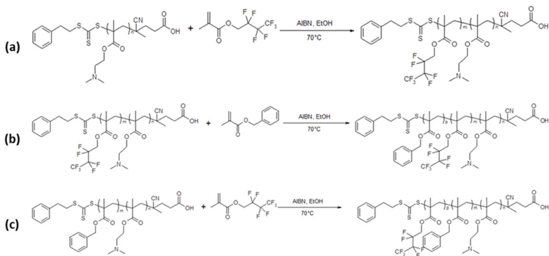
Scheme 1. Sequential RAFT alcoholic dispersion polymerization at 70 °C in ethanol using a poly(2-( N,N ,dimethylamino) ethyl methacrylate) as chain transfer agent of: (a) heptafluorobutyl methacrylate (HFBMA), (b) Benzyl methacrylate (BzMA), (c) heptafluorobutyl methacrylate (HFBMA), resulting in the formations of PDMA-PHFBA and PDMA-PHFBA-PBzMA diblock copolymers ((a,b) respectively), and PDMA-PBzMA-PHFBA triblock copolymers (c).
