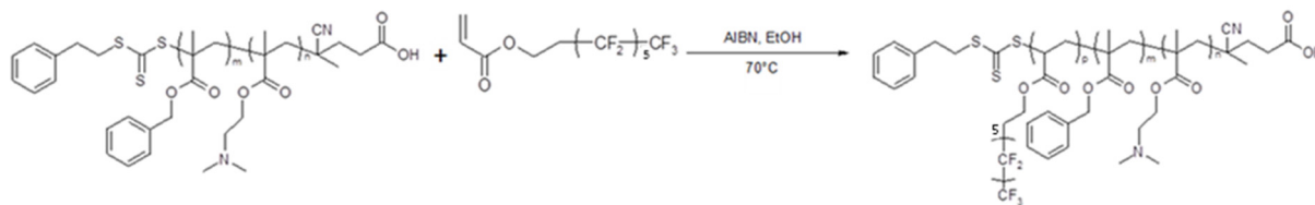
Scheme 2. Synthesis of triblock copolymers prepared by RAFT dispersion polymerization of tridecafluorooctyl acrylate, TDFOA at 70 °C in ethanol using PDMA 58 -PBzMA 198 spherical particles as macroCTA.
