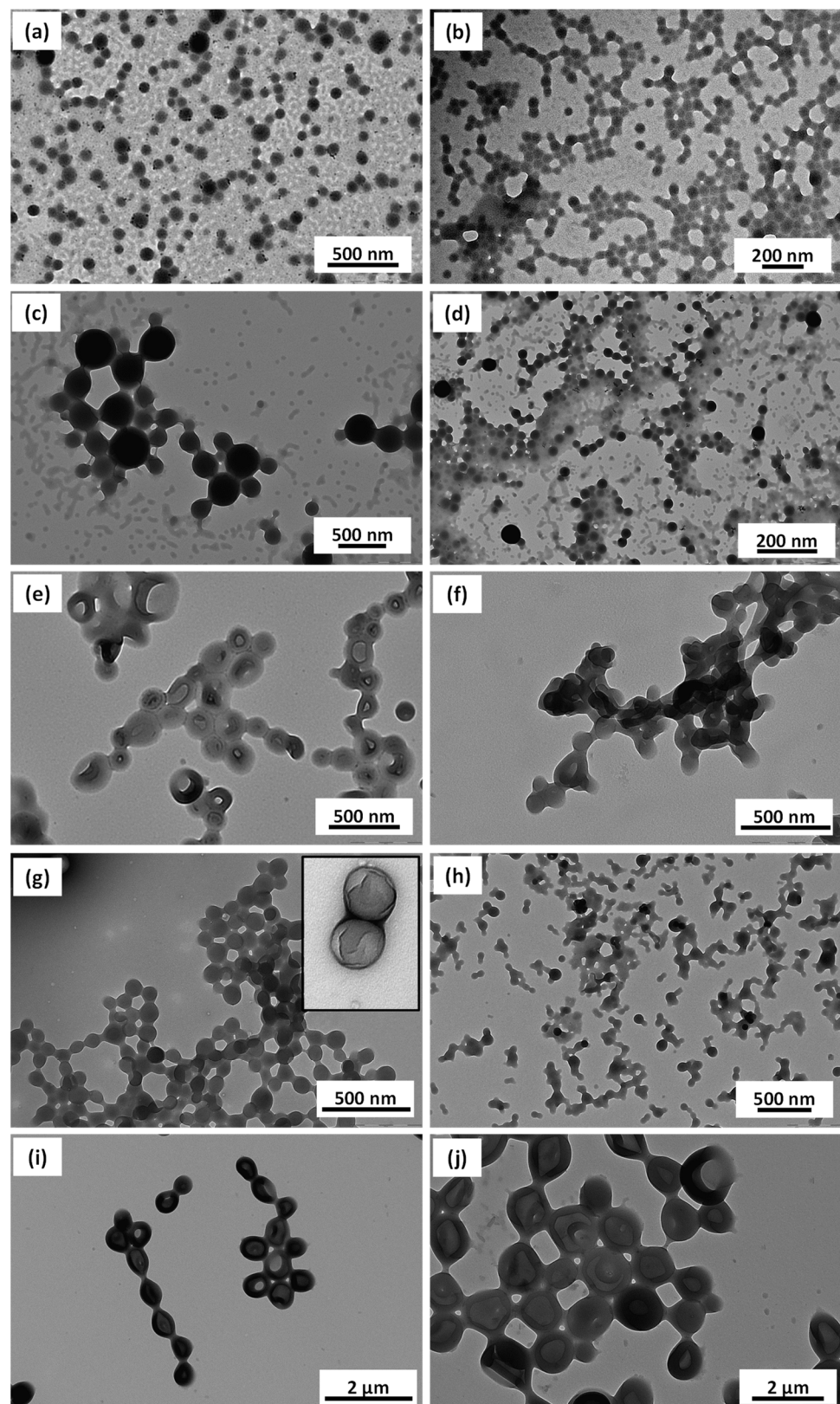
Figure 5. TEM images obtained for PDMA 39 -PBzMA x -PHfBMA y nano objects prepared at 10% w/w with (a) x = 69, y = 50 (b) x = 69, y = 99 (c) x = 69, y = 149 (d) x = 69, y = 196 (e) x = 99, y = 65 (f) x = 149, y = 141 (g) x = 198, y = 50 (h) x = 198, y = 96 (i) x = 198, y = 144 (j) x = 198, y = 189 .
