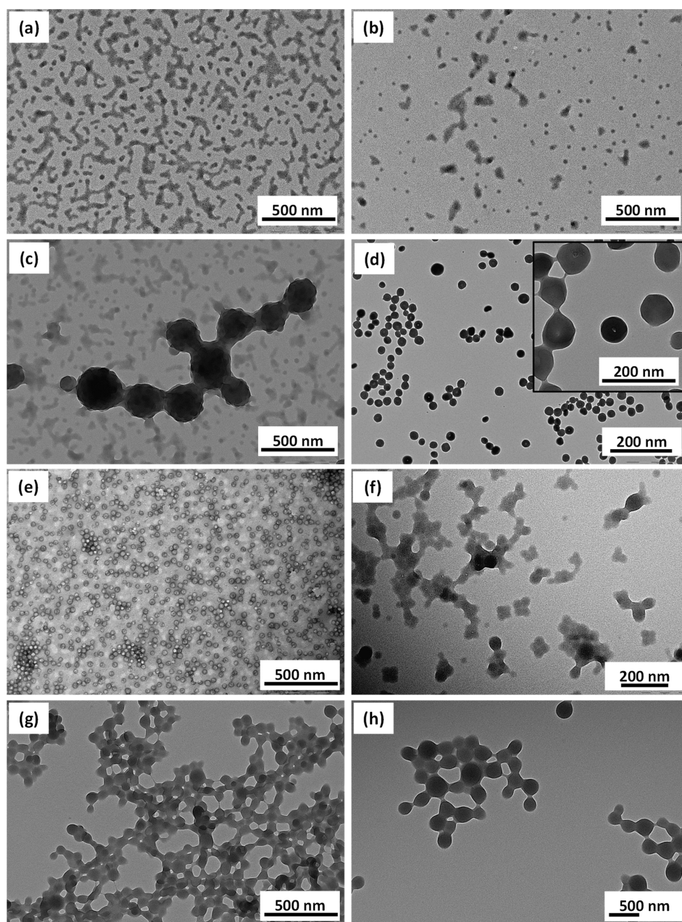
Figure 4. TEM images obtained for \text{PDMA}_{39}\text{-PHFBMA}_x\text{-PBzMA}_y nano objects prepared at 10% w/w with (a) x = 50, y = 69 ; (b) x = 99, y = 69 ; (c) x = 149, y = 69 ; (d) x = 199, y = 66 ; (e) x = 50, y = 198 ; (f) x = 99, y = 198 ; (g) x = 149, y = 198 ; (h) x = 199, y = 198 .
