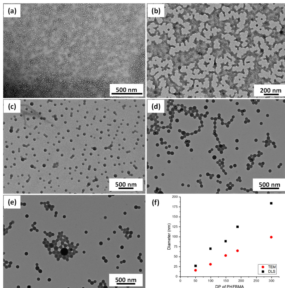
Figure 3. TEM images obtained for PDMA 39 -PHFBMA x nanoobjects prepared at 10% w/w via RAFT alcoholic dispersion polymerization of HFBMA with (a) x = 50, (b) x = 99, (c) x = 149, (d) x = 188, and (e) x = 299. (f) Evolution of the average particles diameter measured by TEM (red dots) and DLS (black squares) with the DP of the PHFBMA core-forming block.
