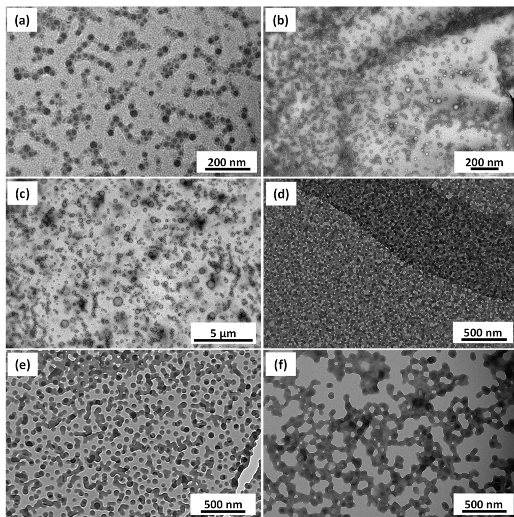
Figure 7. TEM images obtained for PDMA 58 -PBzMA x -PTDFOA y self-assembled nano objects prepared at 10% w/w by RAFT dispersion polymerization of PTDFOA in ethanol, with (a) x = 69, y = 48 (b) x = 69, y = 91 (c) x = 69, y = 144 (d) x = 194, y = 44 (e) x = 194, y = 83 (f) x = 194, y = 120 .
