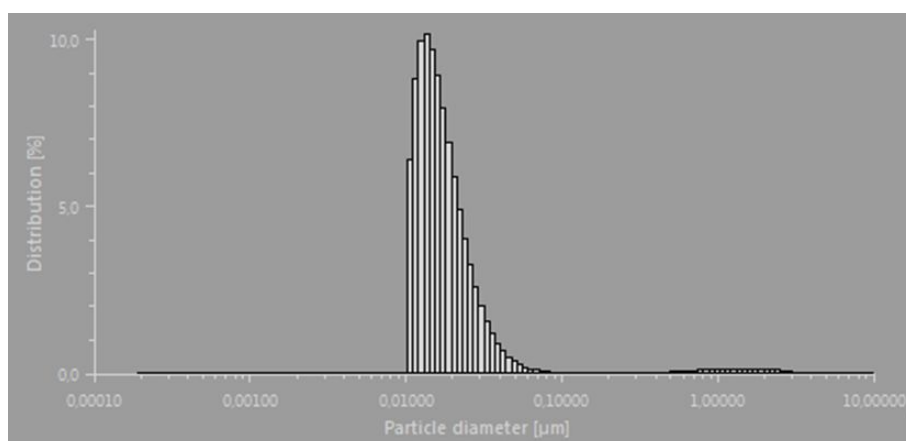
Figure S17. DLS number-average hydrodynamic diameter distribution of \text{CP}(\text{XA})_2 conjugates ( 13.3 \text{ mg mL}^{-1} ) in acetone after heating at 50 \text{ }^\circ\text{C} (20 min) and sonication (20 min).
