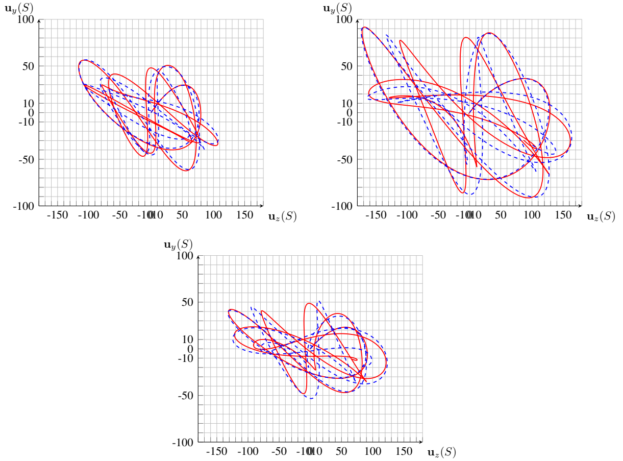
Figure 7: Vertical displacement versus transverse displacement (mm) for S = \frac{L}{4} , S = \frac{L}{2} and S = \frac{3L}{4} , span obtained via FEM (solid line —) and via ROM (dashed line - - -) for a transient dynamics in a nonlinear regime - Parameters are given in Table 3
