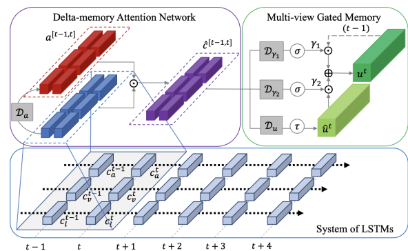
Figure 3: MFN pipeline in [59]
