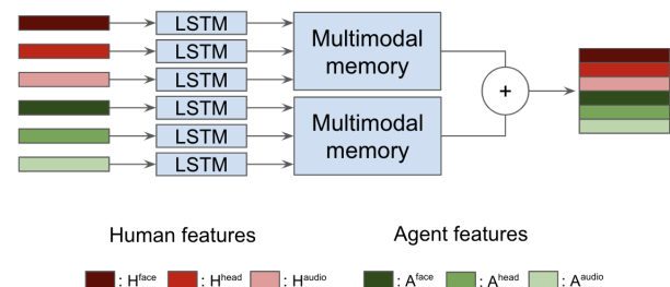
Figure 4: Fusion of multimodal memory cells
