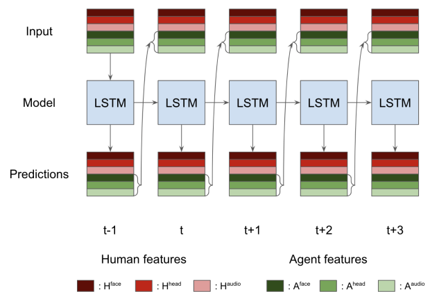
Figure 2: A first model with a symmetrization of the problem
