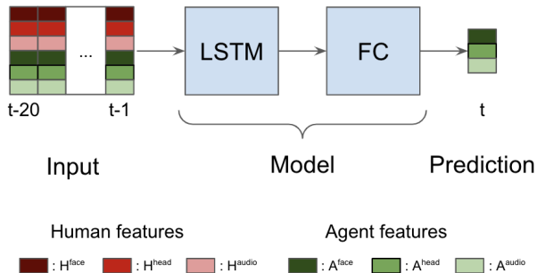
Figure 1: A single LSTM working on a sliding window
