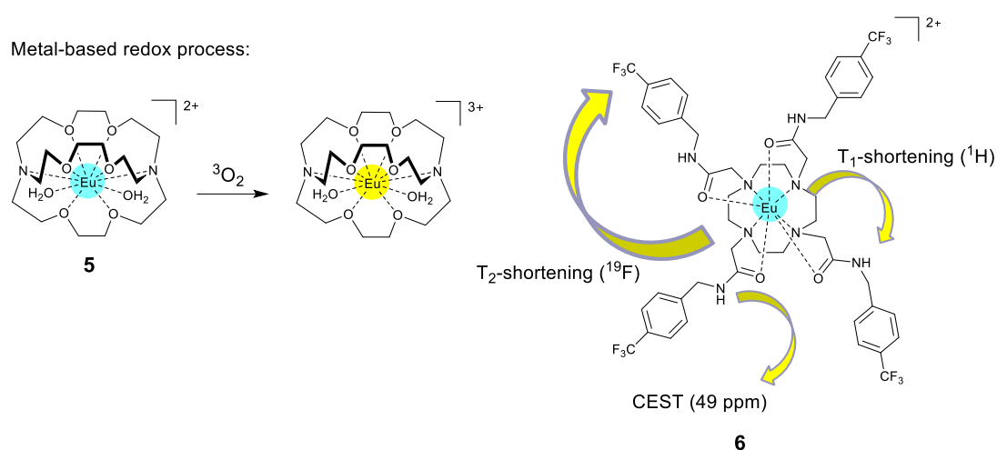
Figure 9. Lanthanide complexes for MRI detection of ^3\text{O}_2
