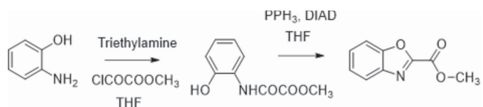
Figure 4 Synthesis route to methyl-1,3-benzoxazole-2-carboxylate.
