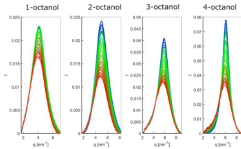
Figure 13: Pre-peaks, as extracted from a procedure explained in section 2
