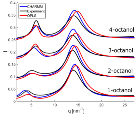
Figure 3: Calculated diffraction patterns (OPLS (red) and CHARMM (blue)) compared to measured data (black).
