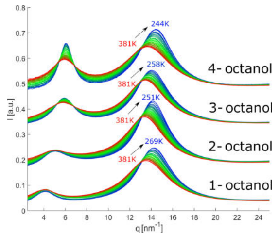
Figure 6: Temperature dependent diffraction patterns of n-octanol ( n=1,2,3,4 ). For visual clarity, the data for the different isomers were shifted vertically.
