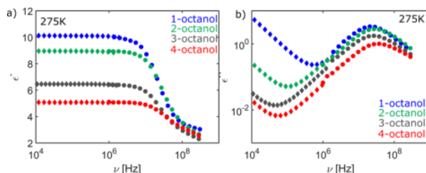
Figure 12: High-frequency (circles) and low-frequency (diamonds) data of the a) real part of the dielectric constant and b) of the loss spectrum for n-octanol (n=1,2,3,4).
