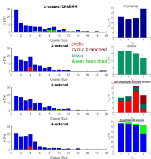
Figure 10: CHARMM Cluster analysis
