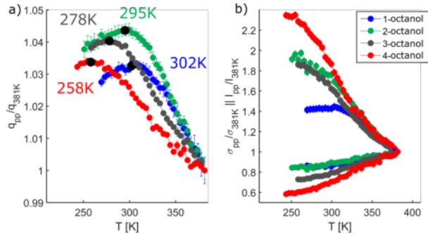
Figure 7: Results of the analysis of the pre-peak. a) Peak position normalized to the position of the maximum temperature. Labeled are the temperatures of the structural crossover (black circle). b) Intensity (diamonds), FWHM (circles) of the n-octanols normalized to the values at 381 K.
