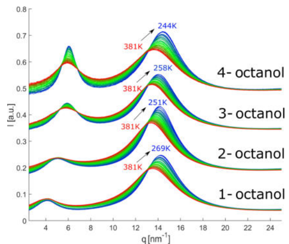
Figure 6: Temperature dependent diffraction patterns of n-octanol ( n=1,2,3,4 ). For visual clarity, the data for the different isomers were shifted vertically.
