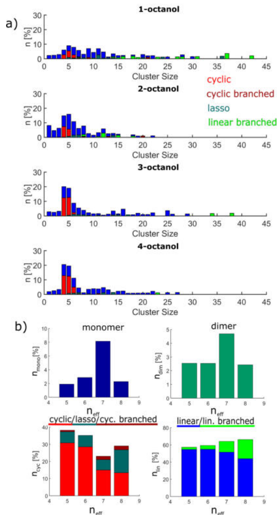
Figure 5: Results of the cluster analysis: a) Overview of the percentage of clusters divided into their sizes. Color coding indicates which structure is present in the cluster. b) Classification of clusters into linear and cyclic structures and into monomers and dimers plotted against n_{eff} .
