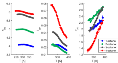
Figure 14: Results of the pre-peak analysis on an absolute scale
