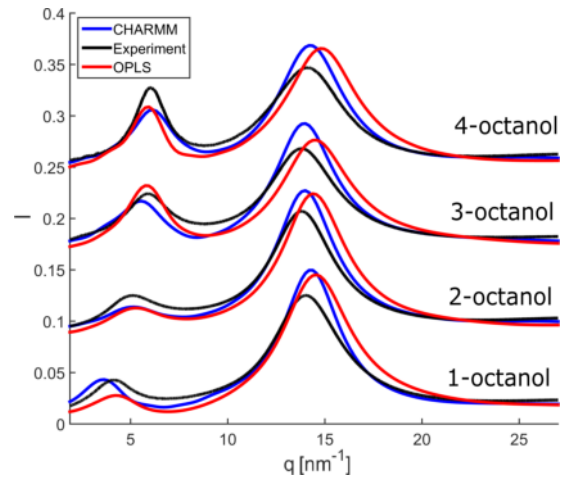
Figure 3: Calculated diffraction patterns (OPLS (red) and CHARMM (blue)) compared to measured data (black).
