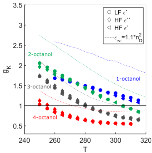
Figure 9: Kirkwood factor of 1-, 2-, 3- and 4-octanol calculated using the low-frequency data via \epsilon' (circles) and using the high-frequency data via \epsilon'' (diamonds) and \epsilon' (triangles). In all cases \epsilon_{\text{inf}} was determined from the high-frequency data via \epsilon' . The dashed lines show the Kirkwood factor calculated using \epsilon_{\infty} instead of \epsilon_{\text{inf}} . The black line marks the structural crossover point.
