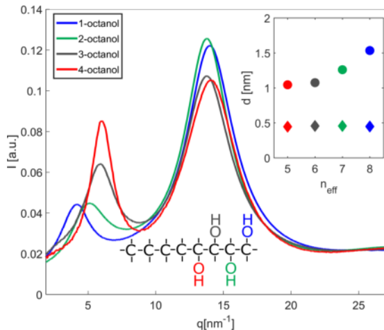
Figure 2: X-ray diffraction patterns of n -octanol isomers with n=1,2,3,4 . The inset displays the supramolecular length scale d = \frac{2\pi}{q_{\text{max}}} obtained from the diffraction pattern plotted against the effective carbon chain length n_{\text{eff}} .
