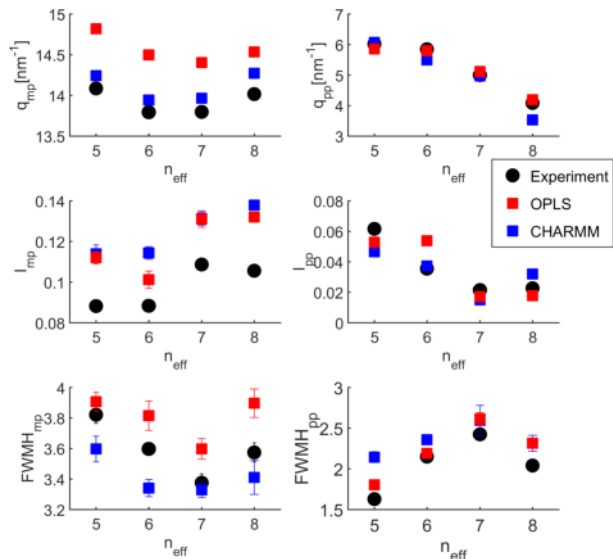
Figure 4: Results of peak analysis of the main peak ( q_{mp} , I_{mp} , FWHM_{mp} ) and the pre-peak ( q_{pp} , I_{pp} , FWHM_{pp} ) emerging from the simulations (OPLS (red) and CHARMM (blue)) are compared to the experimental results (black).
