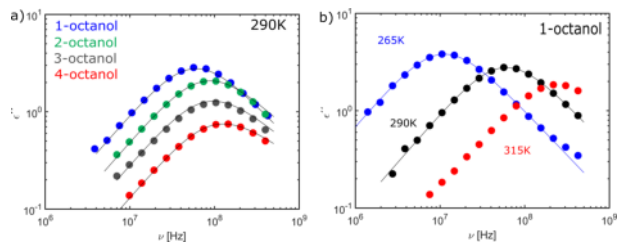
Figure 8: (a) Loss spectra of n-octanol (n=1,2,3,4) measured at a temperature of 290 K, (b) Loss spectrum of 1-octanol at temperatures of 265 K (blue), 290 K (black) and 315 K (red). The solid lines reflect fits using the Cole-Davidson function.
