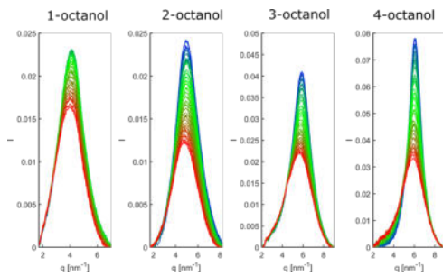
Figure 13: Pre-peaks, as extracted from a procedure explained in section 2
