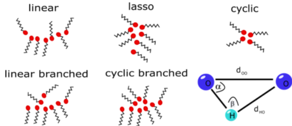
Figure 1: Schematic representation of the OH groups (red circles) forming these classified hydrogen-bonded structures (meta-objects) and the representation of the included distance and angle parameters for cluster analysis.
