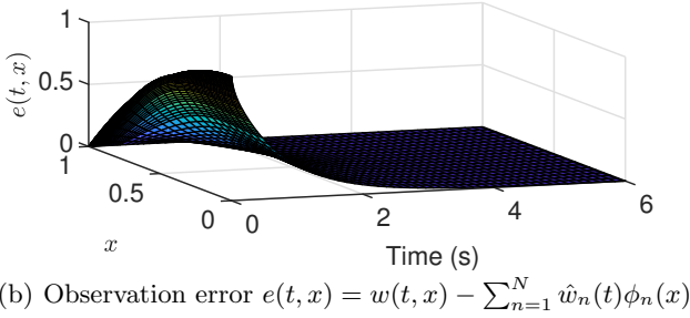
Fig. 1. Time evolution in closed-loop with Dirichlet boundary measurement for the reaction-diffusion PDE (30)
