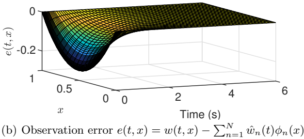
Fig. 2. Time evolution in closed-loop with Neumann boundary measurement for the reaction-diffusion PDE (41)
