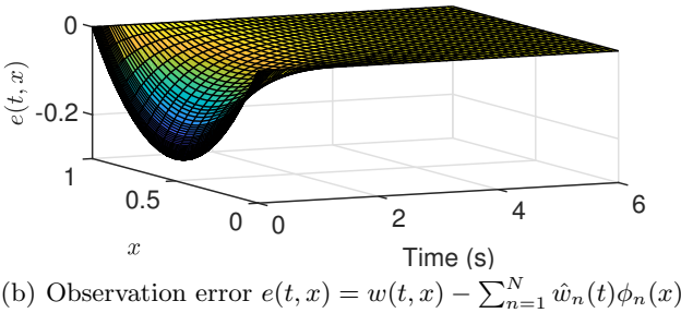
Fig. 2. Time evolution in closed-loop with Neumann boundary measurement for the reaction-diffusion system (41)
