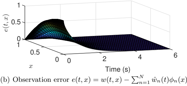
Fig. 1. Time evolution in closed-loop with Dirichlet boundary measurement for the reaction-diffusion system (30)
