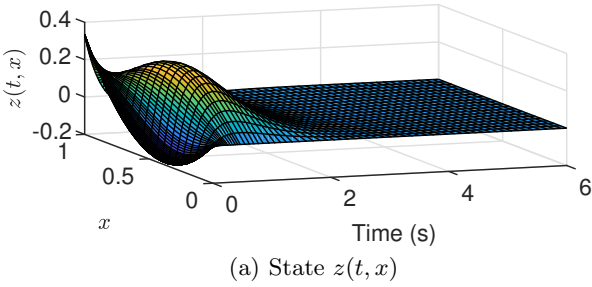
Fig. 1. Time evolution in closed-loop with Dirichlet boundary measurement for the reaction-diffusion system (30)
