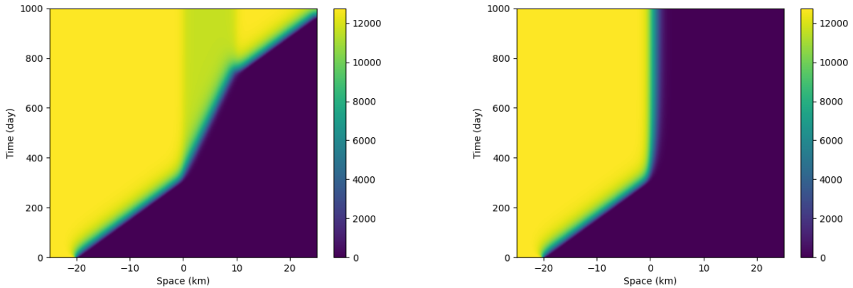
Figure 3: Numerical simulations of system (8)–(9) with L = 10 km and M_0 = 10\,000 \text{ km}^{-2} (left), and M_0 = 30\,000 \text{ km}^{-2} (right).
