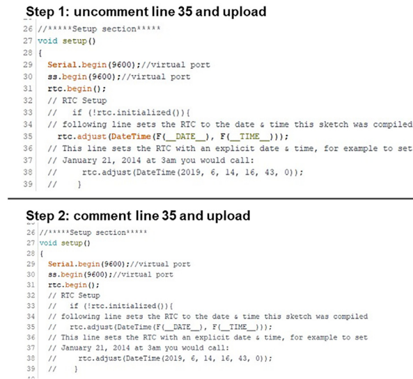
Fig. 7. Two-step procedure to set the RTC time.
