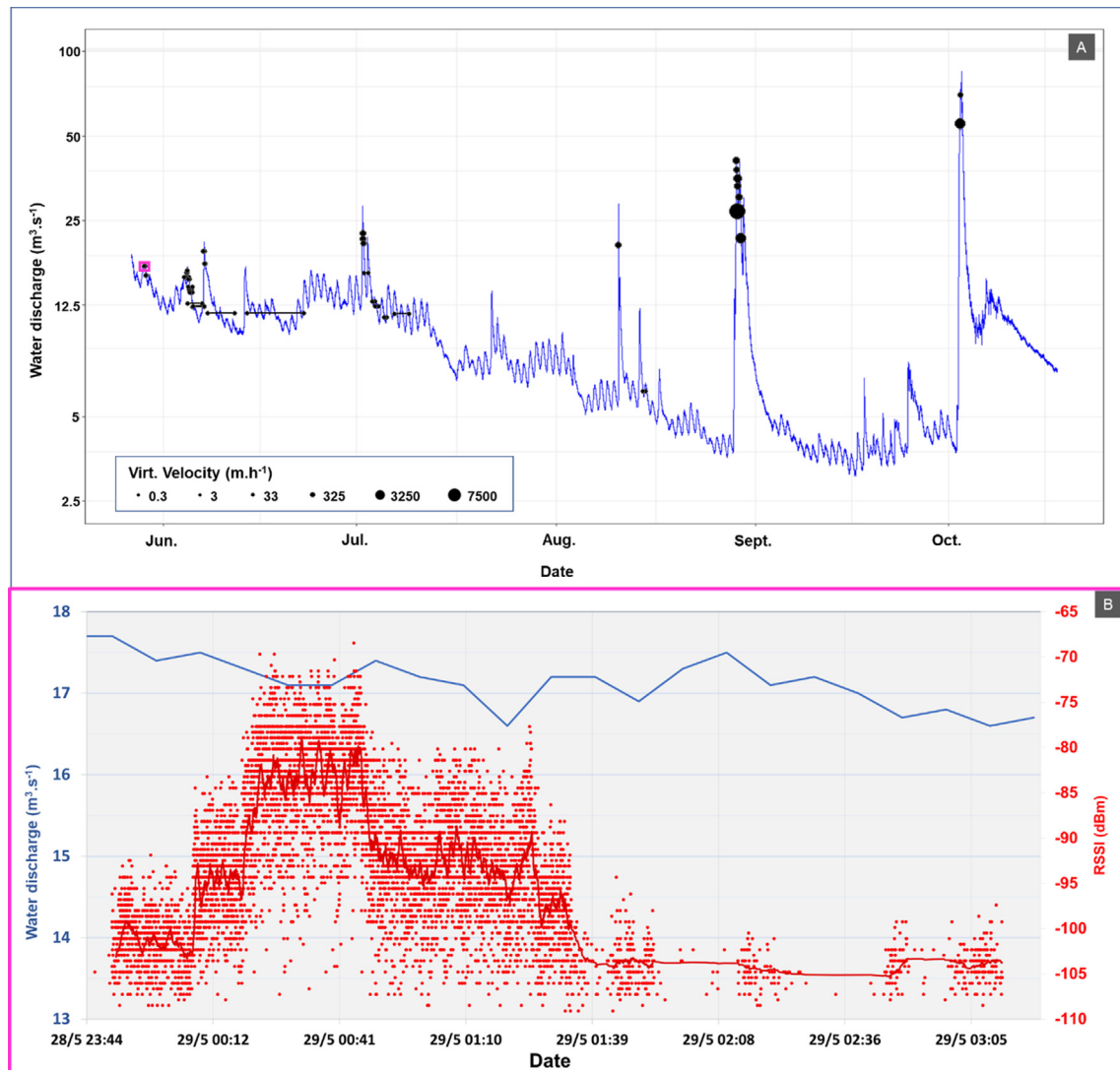
Fig. 11. Example of the monitoring of tracked particle passages during the 2020 field campaign. (A) Date and mean velocity of tracer's passages with regard to water discharge chronic. (B) Focus on a single tracer detailed signal at its passage. Notes: in (A) Black dots indicate timestamp of entry and exit within the antenna sensing field and have a size function of the trace virtual velocity and are scattered at the mean water discharge observed during their passage. Black horizontal lines indicate a long stay within antenna sensing field. Purple square highlight in hydrological chronic the passage of the tracer detailed in (B). In (A) and (B) blue lines indicates water discharge values reported on left-side ordinate axis. In (B) red dots indicate the Received signal strength indication (RSSI) in dBm reported on the right-side ordinate axis of a single beacon signal detection. The red line represents the rolling average in dBm reported on the right-side ordinate axis and based on 100 observations. (For interpretation of the references to colour in this figure legend, the reader is referred to the web version of this article.)
