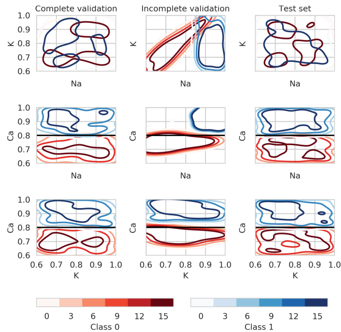
FIGURE C.3. Section 4.2.3: Densities of validation and test sets for calcium channel blockade classification. Black lines correspond to the class delimitation.
