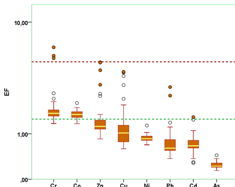
Figure 3. Enrichment factor of trace element in sediments from the Sebou basin normalized to the Tafna bedrock [29]. The upper outliers (above 1.5) are for stations S3, S4 and A1. Mostly the orange circles indicate the Fez station (S3).. The dash lines green and red indicate EF value of 1,5 and 5, respectively.
