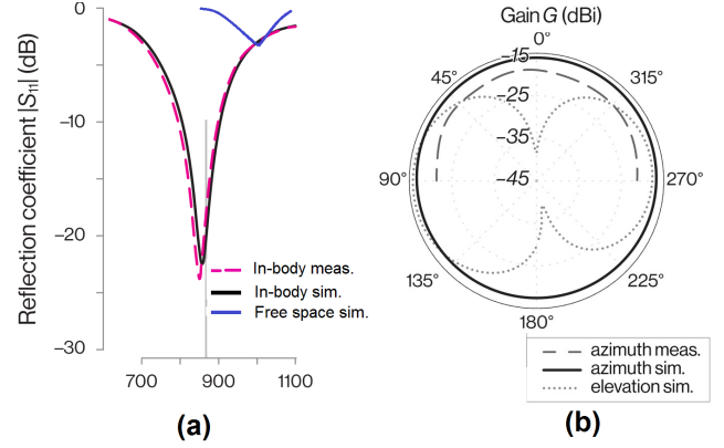
Fig. 2. (a) The reflection coefficient |S_{11}| in free space and in a phantom (in-body) with muscle-equivalent EM properties. (b) In-body measured and computed radiation patterns.
