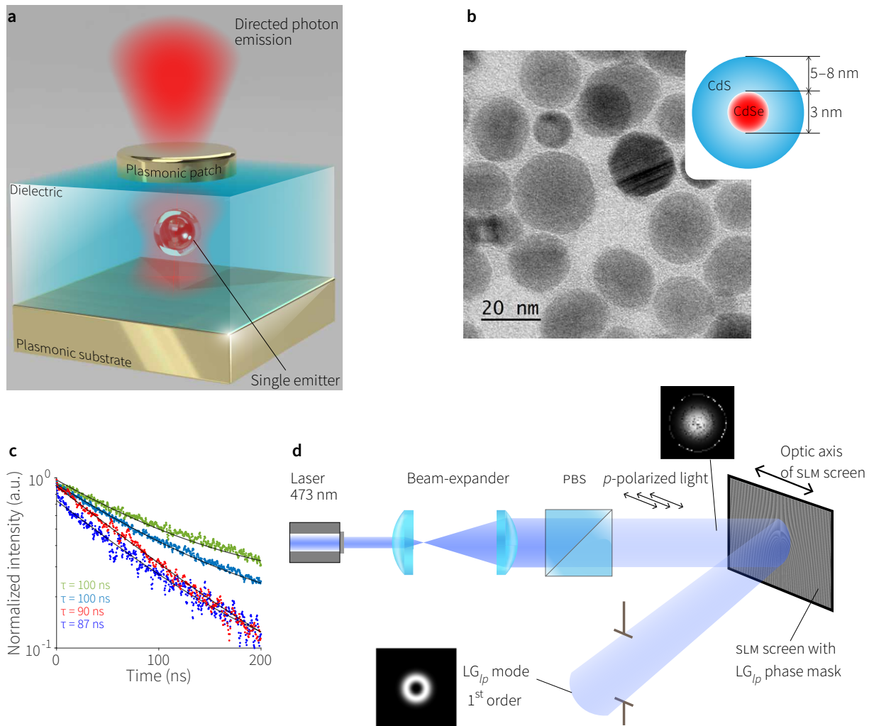
Figure 1 Single-emitter plasmonic patch antenna with a QD
