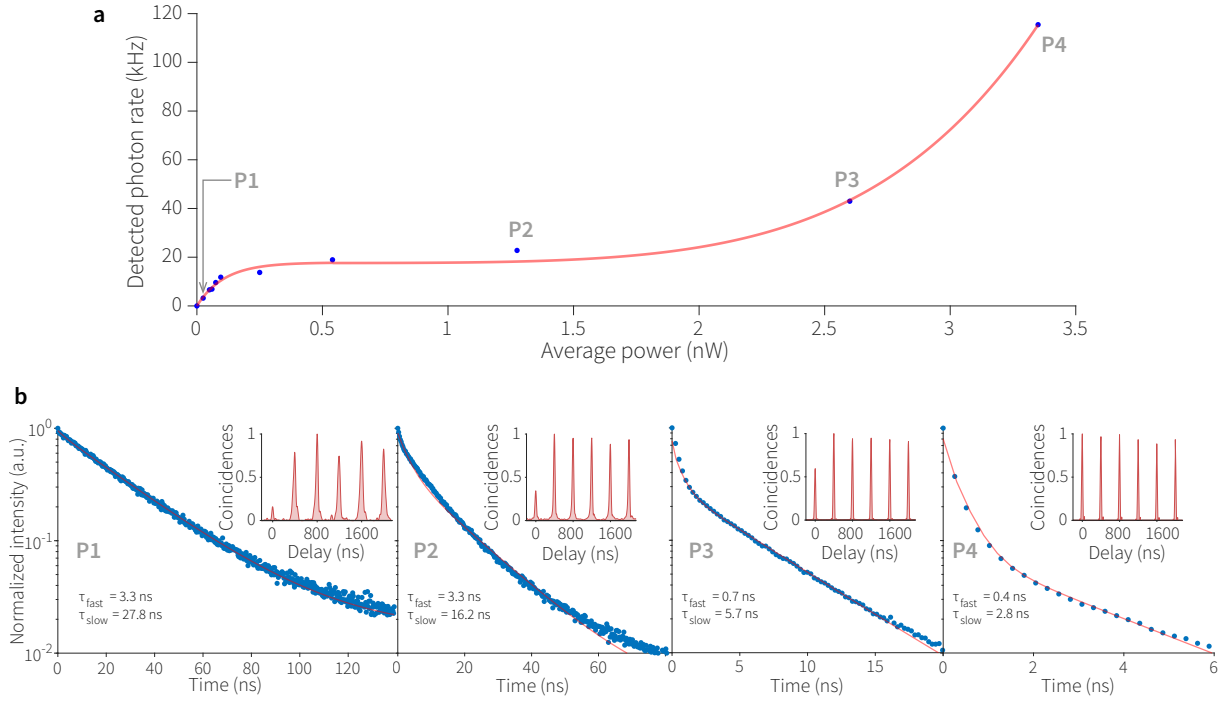
Figure 5 Excitation and multiexciton emission in plasmonic antenna
