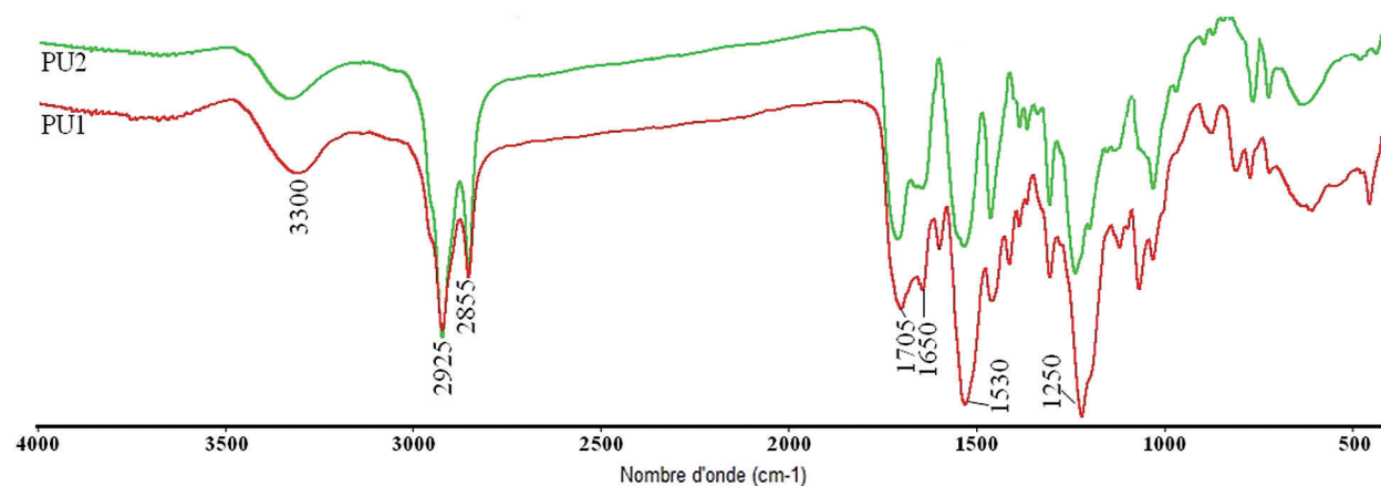
Figure 5: FTIR spectrum of PU1 and PU2
