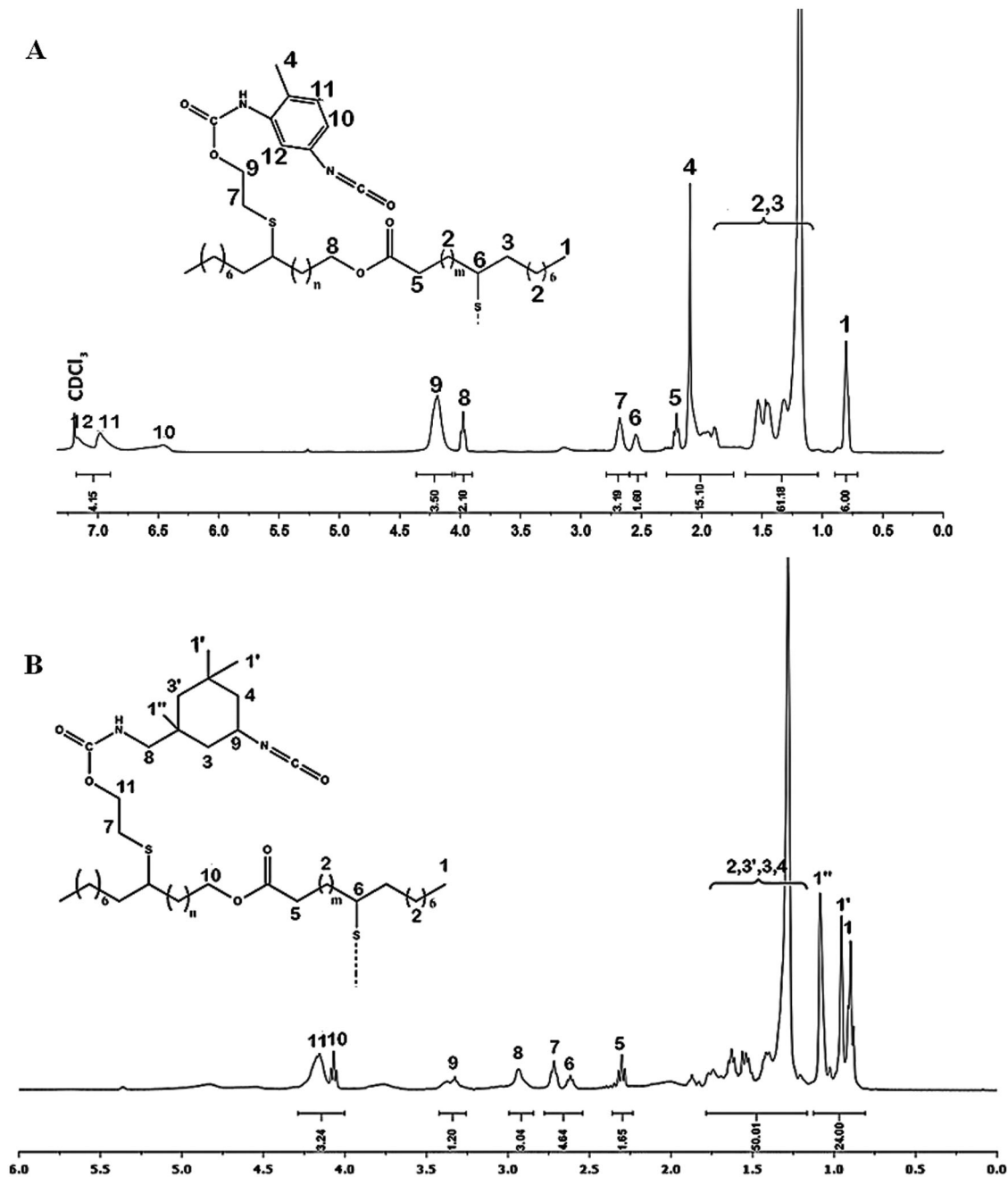
Figure 4: NMR spectrum of (A) Pr1 and (B) Pr2 in CDCl 3
