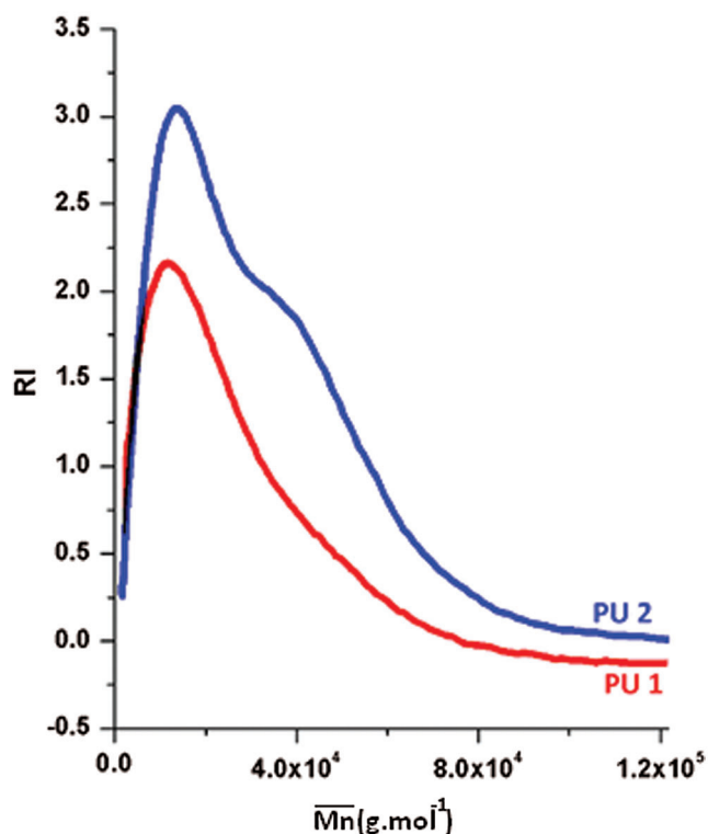
Figure 8: GPC curves of PU1 and PU2
