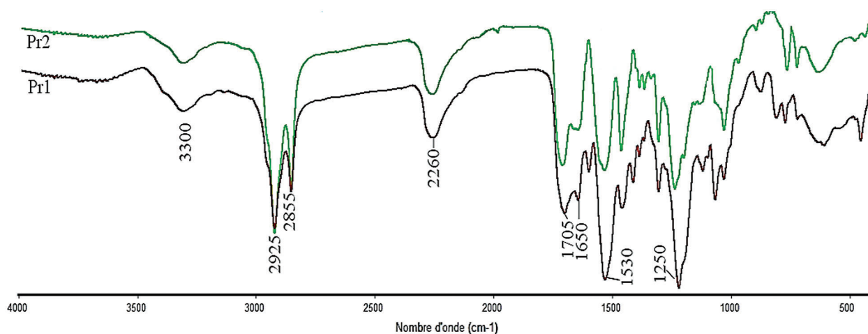
Figure 3: FTIR spectra of Pr1 and Pr2
