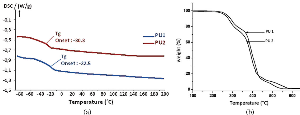
Figure 7: DSC (a) and TGA (b) curves of PU1 and PU2
