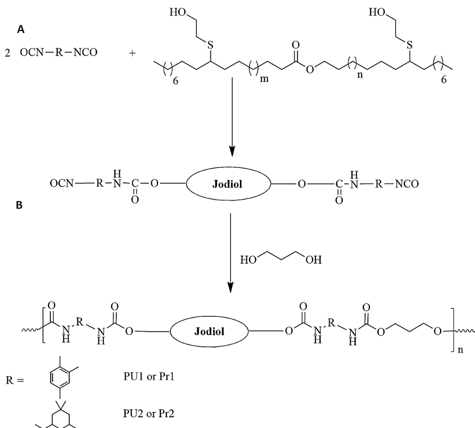
Figure 2: (A) Synthesis of prepolymers and (B) Synthesis of final PU materials
