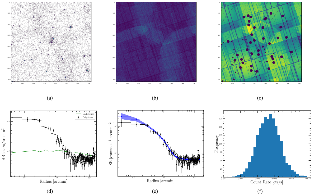
Fig. A.1. Example of cluster count-rate measurement with the pyproffit method. The displayed cluster is XLSSC 093 at a redshift of 0.429. (a) X-ray mosaic around the cluster; the image is 30 arcmin aside. (b) Particle background map. (c) Combined exposure map along with the masks hiding the neighbouring sources. (d) Extracted cluster profile (black crosses); the green line displays the particle background level extracted from map (b); this component is already subtracted from the displayed profile. (e) Overlaid on the extracted profile, the reconstructed (PSF-deconvolved) profile is shown in blue along with the 1- \sigma estimated uncertainty. (f) Count-rate posterior distribution (MOS1 normalised) of the reconstructed profile.
