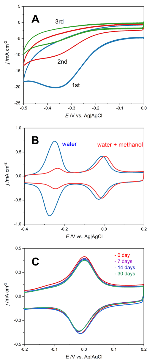
Figure 1. (A) Cyclic voltammograms for the reduction of ca. 5 mM azure A diazonium recorded at a scan rate of 0.1 \text{ V s}^{-1} in 0.25 M HCl and 10 mM NaNO 2 as the supporting electrolyte; the first three cycles are shown: 1st (blue), 2nd (red) and 3rd (green). (B) Cyclic voltammograms of an Azure A-modified MWCNT electrode washed with water (blue), followed by methanol (red), in phosphate buffer (pH 7.0) at a scan rate of 10 \text{ mV s}^{-1} . (C) Stability testing of an Azure-A-modified MWCNT electrode after washing with methanol by recording cyclic voltammograms in phosphate buffer (pH 7.0) at a scan rate of 10 \text{ mV s}^{-1} after 0 (red), 7 (purple), 14 (blue), and 30 d (green). The electrodes were stored in a refrigerator in phosphate buffer (pH 7.0) at 4^\circ \text{C} until used.
