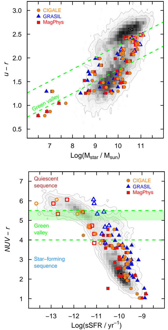
Fig. 14. Colors of KINGFISH galaxies plotted against the logarithm of stellar mass given by the respective SED-fitting algorithms ( top panel ) and the SED-derived logarithm of sSFR ( bottom , with units of \text{yr}^{-1} ); the top panel shows SDSS u-r , and the bottom \text{NUV}-r . In both panels, the KINGFISH galaxies are superimposed on the GSWLC sample, taking only those galaxies with 0.015 \leq z \leq 0.06 . As in previous figures, filled symbols correspond to high specific SFR ( \text{Log}(\text{sSFR}/\text{yr}^{-1}) > -10.6 ), and open ones to low specific SFR ( \text{Log}(\text{sSFR}/\text{yr}^{-1}) \leq -10.6 ). In the top panel , the (green) dashed lines correspond to the separation of the “green valley” from the upper (red) and lower (blue) loci of SDSS galaxies as given by Schawinski et al. (2014). In the bottom , we have included the \text{NUV}-r color range for the “green valley” transition proposed by Salim (2014), together with the limit for ETG SF activity of \text{NUV}-r = 5.5 given by Kaviraj et al. (2007). The green shaded area marks the (uncertain) boundary between star-forming and quiescent ETGs.
