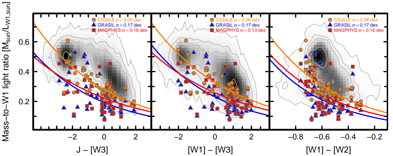
Fig. 20. Mass-to-light ratios in the WISE W1 band of KINGFISH galaxies plotted vs. the J-[W3] color ( left panel ); [W1]-[W3] ( middle ); and [W1]-[W2] ( right ). As in Fig. 19, the underlying gray scale corresponds to the GSWLC data (Salim et al. 2016). Legends in the upper right corners give the rms deviation of the robust best fits, shown as curves in each panel, of the M/L(W1) ratios vs. and colors. The best fit rms of 0.05 dex (for CIGALE) is obtained for M/L as a function of J-[W3] ( left panel ), but [W1]-[W3] is only 0.01 dex worse (for CIGALE, see middle panel ). The fit of M/L with [W1]-[W2] ( right panel ) is the worst of all three colors shown here, but only by 0.03 dex (for CIGALE, comparable for the other two algorithms). All magnitudes are on the AB system.
