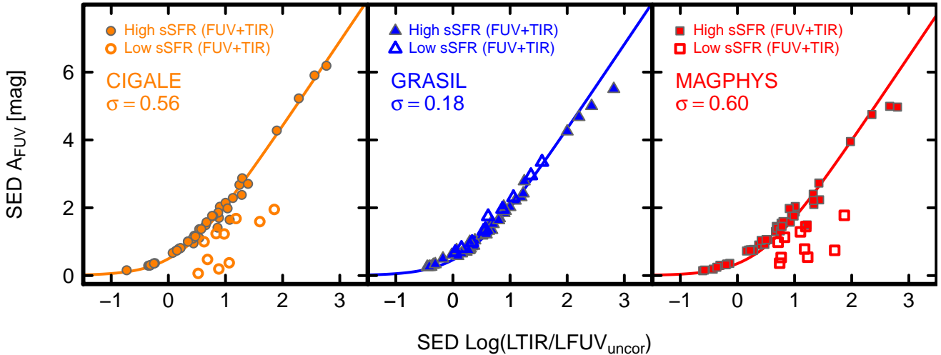
Fig. 10. SED-derived A_{FUV} plotted against SED-derived IRX [\log_{10}(L_{TIR}/L_{FUV})] . The solid curve shows the fit obtained by adopting the formulation in Eq. (7); as described in the text, the best-fitting a_{FUV} values are estimated using only the galaxies with (\text{Log}(\text{sSFR}/\text{yr}^{-1}) > -10.6) . The mean deviations comparing the SED-derived A_{FUV} and the fitted ones from SED-derived IRX (now including all galaxies) are shown by the \sigma value in each panel. As in previous figures, filled symbols correspond to high specific SFR ( \text{Log}(\text{sSFR}/\text{yr}^{-1}) > -10.6 ), and open ones to low specific SFR ( \text{Log}(\text{sSFR}/\text{yr}^{-1}) \leq -10.6 ), as noted in the legend in the upper left corners.
