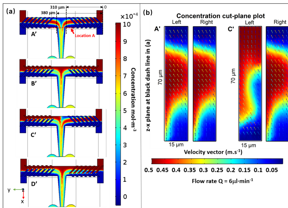
Figure 3. Simulation results along the mixing channel of four SHB designs A', B', C', D'. (a) shows the concentration profiles in the x - y plane at z=7.5 \mu\text{m} (middle of the channel), the two black dashed lines indicate the locations at the end of premixing after passing through half cycle of the grooves on each side (distance of 310 \mu\text{m} and 380 \mu\text{m} from the entrance at the right), while the red dashed line indicates the location where the combined solutions change the flow direction to x . (b) is the slice concentration profile projected onto x - z plane located at the black dashed lines at 310 and 380 \mu\text{m} from the right channel labelled as “left” and “right”, respectively. The concentration profile shares the same color bar with (a). Velocity vectors were plotted as colored arrows with the color bar representing the velocity ( \text{m}\cdot\text{s}^{-1} ). The simulations were performed with the COMSOL Multiphysics software ( http://www.comsol.com ).
