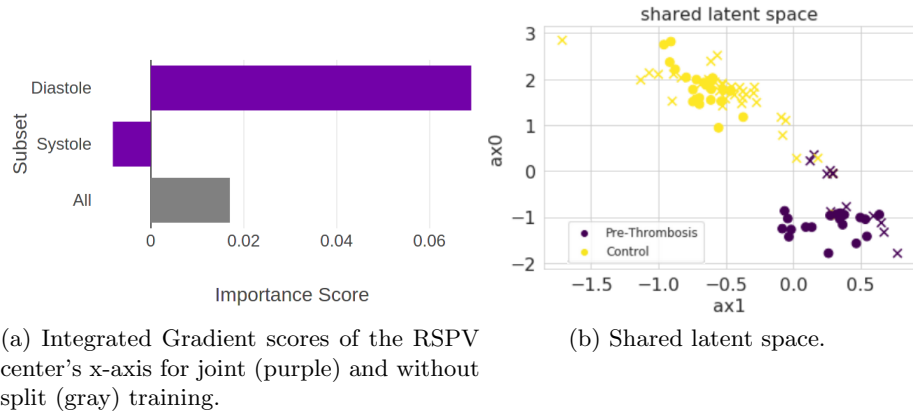
Fig. 4. Results of the method. Joint analysis enables better interpretation of biomarkers (4a) as well as successful representation in the latent space (4b).
