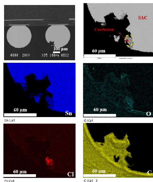
Fig. 4. EDX of as-received BGA sample solder ball (5% NaCl at 35°C) after 48h in salt spray chamber
