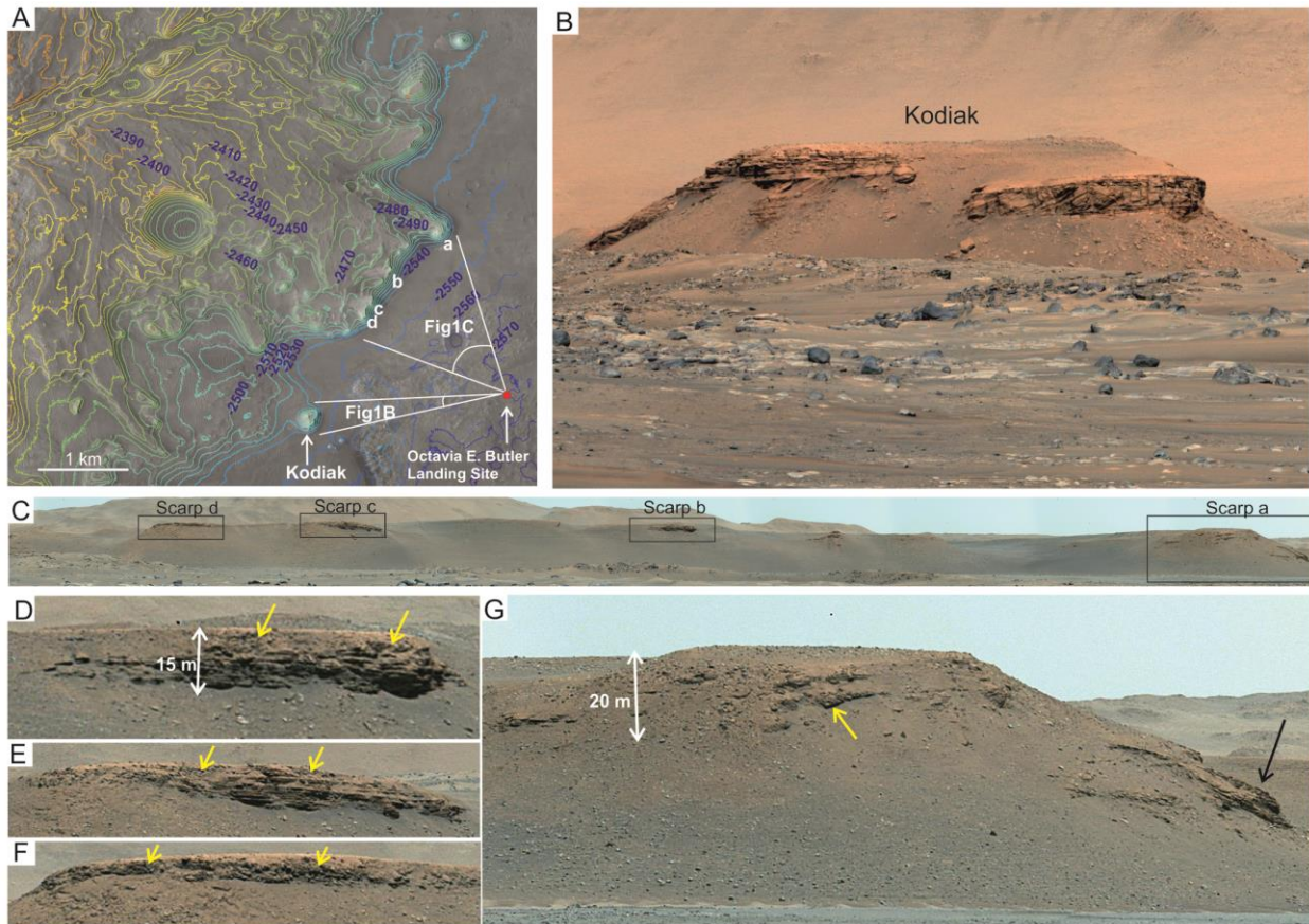
605 Figure 1: Orbital and rover context observations of the Jezero crater western fan. (A) High Resolution Imaging Science Experiment (HiRISE) mosaic ( I4 ) with 10 m elevation contours from a digital elevation model (DEM) ( I4 ) showing the western fan inside Jezero crater and the landing site, informally named the Octavia E. Butler (red dot). White arcs represent the field of view of 610 Fig. 1B and 1C. (B) The butte informally named Kodiak was imaged from a distance of ~2.24 km by Mastcam-Z. (C) Mastcam-Z enhanced color mosaic of the delta front, taken from a ~2.20 km distance with close-ups on scarps of interest (a to d). (D-G) Each scarp is imaged by the corresponding 110 mm focal length Mastcam-Z images. Yellow arrows indicate the location of 615 boulder-rich material shown in Fig. 3-4. The black arrow in (G) indicates an exposure with dipping strata.
