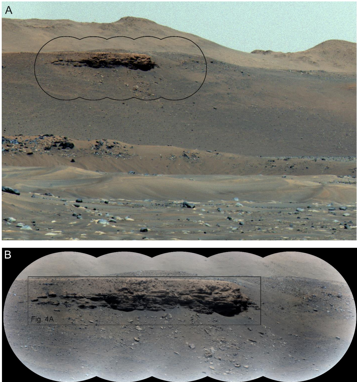
Figure S4: Images of the delta front, scarp b. (A) Mastcam-Z left-camera enhanced color stretch image of delta front scarp b (see Fig. 1) with footprints of the SuperCam RMI mosaic. (B) SuperCam RMI mosaic with enhanced stretch color. See Tab. S1 and S2 for more details.
