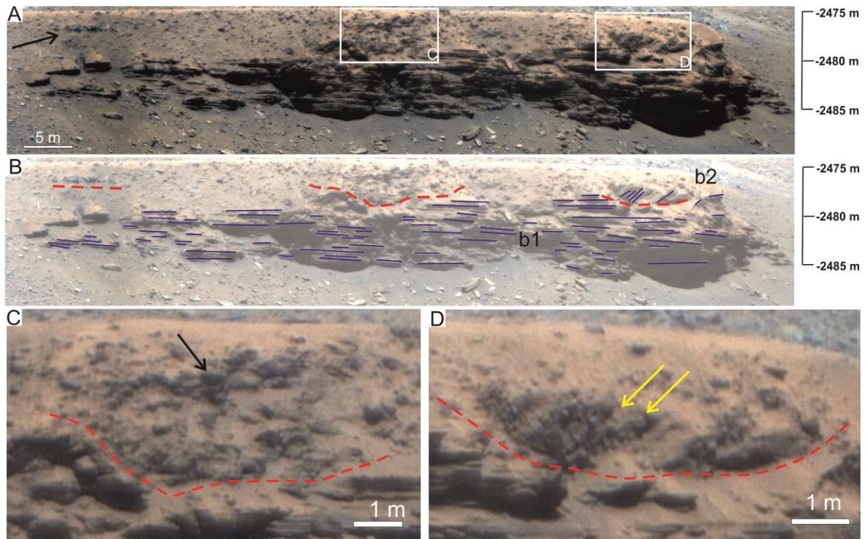
Figure 4: Stratigraphy of the western fan scarp b. (A) Mosaic of five RMI frames of scarp b (localization in Fig. 1, mosaic in Fig. S4). The black arrow at the top left indicates a thin bed with cobbles and boulders preserved in the scarp similar to the thinning of a2 in Fig. 3. Elevations scales are as in Fig. 2. White boxes indicate regions shown in more detail in other panels. (B) Line drawing interpretation of this scarp, showing individual beds (blue lines) and discontinuities (dotted red lines). Sub-horizontal beds dominate the lower sedimentary unit b1. This unit displays a relatively fine-grained material compared to overlying boulder-bearing conglomerates b2, which are present above a discontinuity (dashed red lines) interpreted as a truncation episode. (C) Zoomed image of a boulder conglomerate displaying a series of rounded boulders, piled up along a sub-horizontal bed, 50 cm to 1 m in diameter, developed along a sub-horizontal bed (black arrow). (D) Zoomed image of cobble-bearing conglomerates that were deposited as dipping beds (yellow arrows). The presence of bedding indicates the conglomerate exposure is not a residual lag lying on hillslopes.
