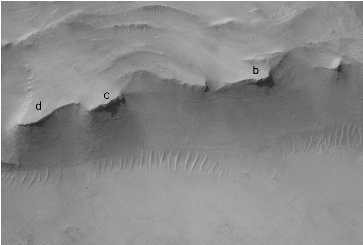
Figure S5: Entry, Descent and Landing (EDL) camera image of the delta front taken during the descent. The image highlights the talus and the presence at a similar elevation of three of the scarps that have subsequently been observed from the ground (Fig. 1, S4). Scarp b is approximately 15 m high and 70 m long and was the focus of the RMI mosaic (Fig. 4 and S4) while scarps c and d have been observed by Mastcam-Z only (Fig. 1). Orientation of the top of the image toward northwest. Image number RDC_00000005_000_003893_raw.
