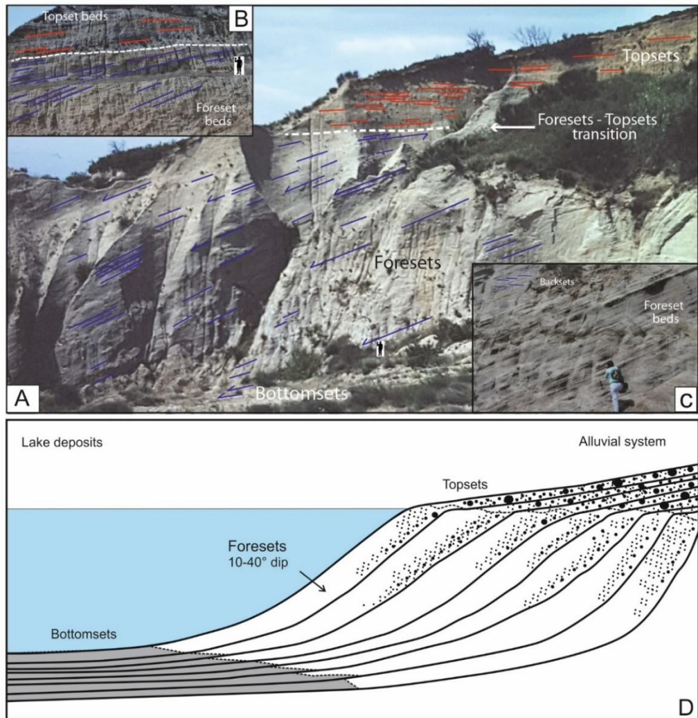
1075 Fig. S8. Geometry of Gilbert-type fan deltas. (A) General view of the Pliocene of Bente Farine Quarry, Néfiach 1080 area, Pyrénées-Orientales, France (images taken in 1993) showing a Gilbert delta with the typical tripartite structure 1085 of a Gilbert fan delta (topsets, foresets, bottomsets) marked by depositional slopes that dip steeply (general linear slope of 22^\circ to the left). The section shown is subparallel to the direction of progradation and the vertical development of the foreset section is approximately 25 m (human silhouette for scale). (B) Topset beds consisting of crudely stratified, gently inclined floodplain to soil heterolithic deposits and sheetflood to braided river conglomerates. The topset–foreset boundary is transitional, producing a sigmoidal stratal termination pattern. The toplap-type foresets– topsets surface marks the transition from marine (foresets) to continental (topsets) depositional facies. (C) Coarse- grained foresets with well-defined bedding and steep primary dips to the left ( 22^\circ ). The (lower slope) foreset beds have a mostly planar geometry, with high lateral persistence. They are composed of coarse sandstones and resistant, clast-supported, poorly-sorted pebbly sandstones. Note sets of upslope-dipping cross-strata that occur as thin, sub- horizontal sand beds. (D) Sketch of a Gilbert delta on Earth (after 19). To the right, a fluvial system (coarse material, topsets) transitions gradually into steeply inclined foresets with locally coarse, generally finer-grained material, which transition into bottomsets comprising only fine-grained material (mudstones, in gray tone) at the lake bottom.
