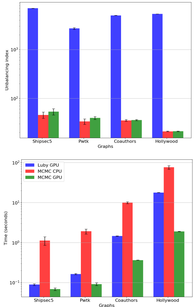
Figure 2: Average unbalancing index (upper plot) of final colorings achieved by the three algorithms for the graphs of Table 1 and related average execution times (lower plot), expressed in seconds. Results are on 35 repetitions (standard deviation as error bar) and plotted in logarithmic scale.
