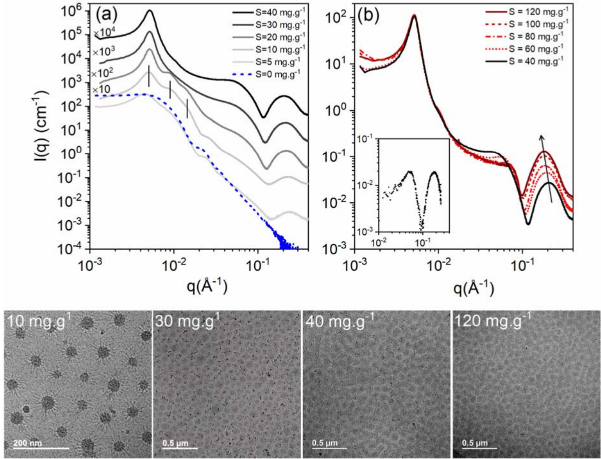
Figure 7. Microstructure of nanocomposites investigated by SAXS ((a) and (b)) and cryo-TEM micrographs (below); C = 25 \text{ mg.g}^{-1} . In (a) the curves for S = 10, 20, 30, and 40 \text{ mg.g}^{-1} are shifted vertically by a factor 10, 10^2, 10^3, and 10^4 respectively. In (b) the inset shows the SAXS intensity scattered by a pure SDS solution in water ( S = 20 \text{ mg.g}^{-1} ); the upturn of the intensity at low q values signals the emergence of attractive interactions.
