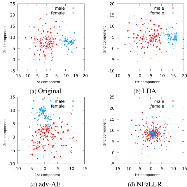
Fig. 2: UMAP visualisation (with euclidean metric and 30 neighbors) [22] of the original and protected V2T’s x-vectors. Even with the LDA and adversarial based methods, unsupervised visualisation allows separation of the sex while with the proposed approach, male and female x-vectors are mixed.
