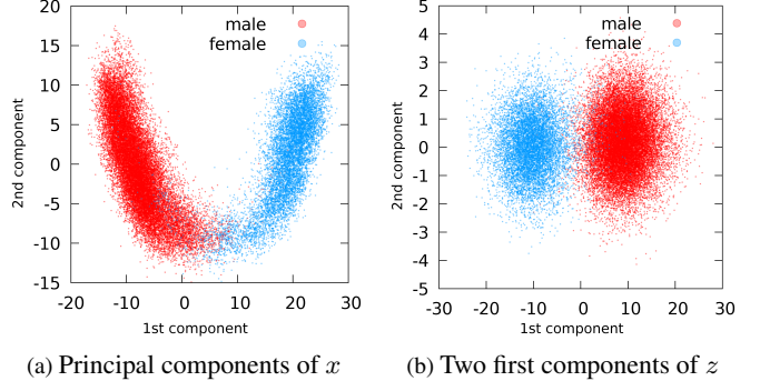
Fig. 1: V2T’s x-vectors visualisation in the original and latent space. In the latent space (b), class-conditional densities are Gaussian and only the first component is discriminant while this is not the case in the original feature space (a).
