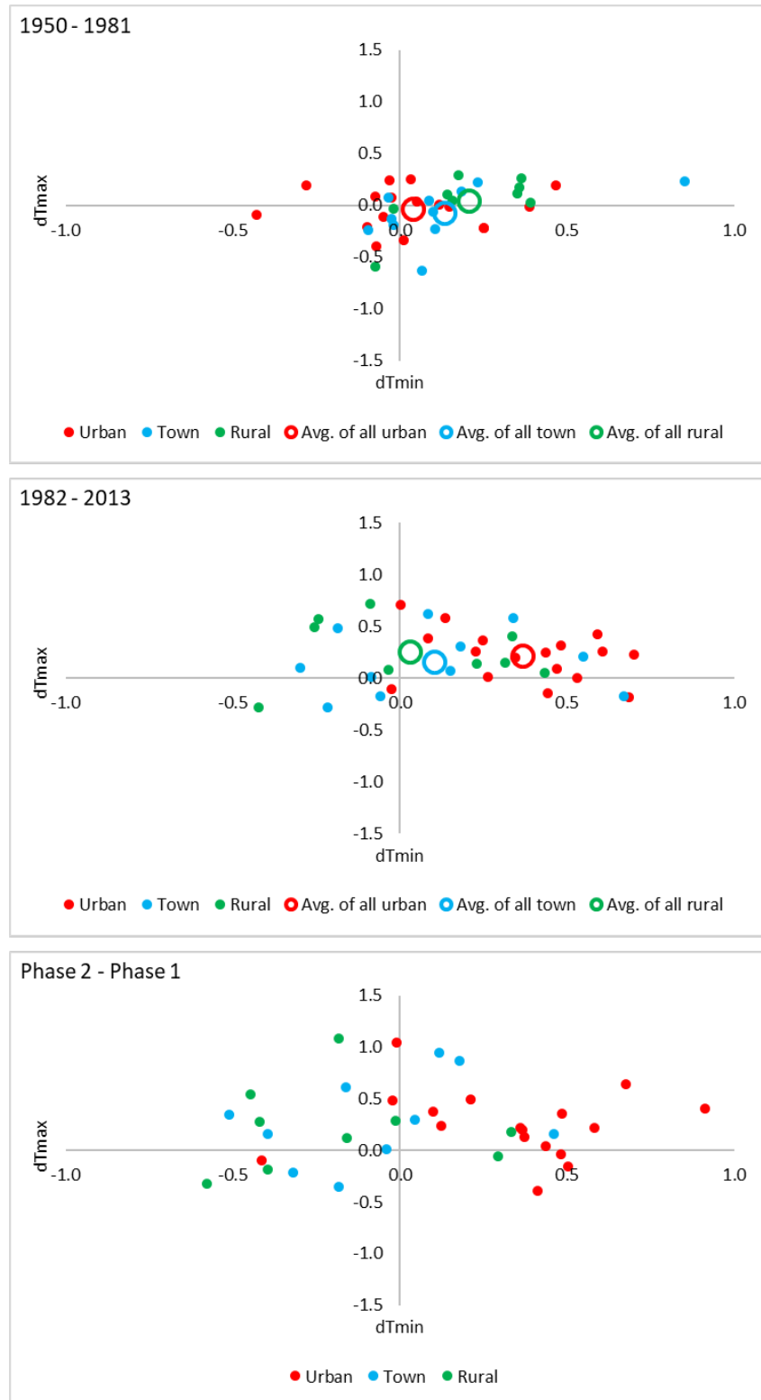
Figure 4: Per decade change in trends of dT_{\min}^a (x-axis) as a function of trends of dT_{\max}^a (y-axis) for urban (red filled circles), town (blue filled circles) and rural (green filled circles) stations for P1 (a); P2 (b) and dT_{P2-P1} (c). The hollow red, blue and green circles in a (P1) and b (P2) represent the trends of dT_{\min}^a as a function of trends of dT_{\max}^a drawn by taking the mean of all urban, town and rural stations, individually, respectively.
