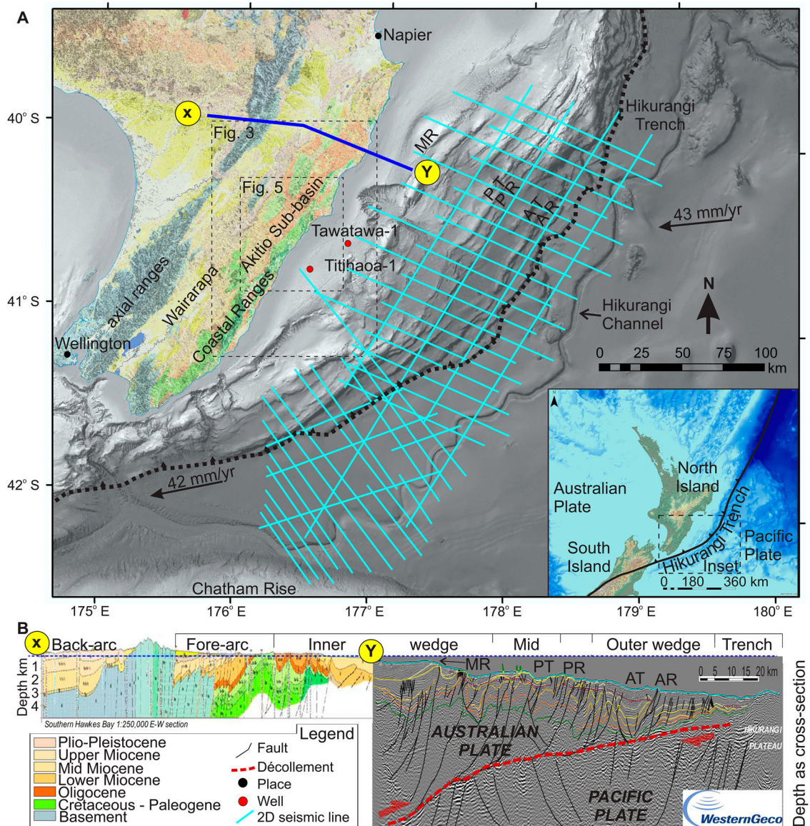
Figure 1. A, Hikurangi Margin onshore geological map (Heron 2014) and offshore bathymetry (courtesy of NIWA). B, Integration of geological cross section (modified from Lee and Begg 2002) and interpreted, depth migrated seismic line courtesy of WesternGeco, both at same vertical and horizontal scale, with \times 4 vertical exaggeration. AT = Akaitio Trough; AR = Akaitio Ridge; MR = Motuokura Ridge; PT = Porangahau Trough; PR = Porangahau Ridge.
