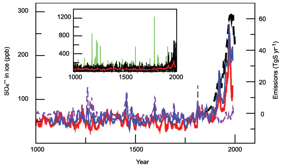
Figure 6.15. Sulphate ( SO_4^{2-} ) concentrations in Greenland (Bigler et al., 2002, red line; Mieding, 2005, blue) and antarctic (Traufetter et al., 2004, dash, violet) ice cores during the last millennium. Also shown are the estimated anthropogenic sulphur (S) emissions for the NH (Stern, 2005; dashed black). The ice core data have been smoothed with a 10-year running median filter, thereby removing the peaks of major volcanic eruptions. The inset illustrates the influence of volcanic emissions over the last millennium and shows monthly sulphate data in ppm as measured (green), with identified volcanic spikes removed (black, most recent volcanic events were not assigned nor removed), and results from the 10-year filter (red) (Bigler et al., 2002). The records represent illustrative examples and can be influenced by local deposition events.
