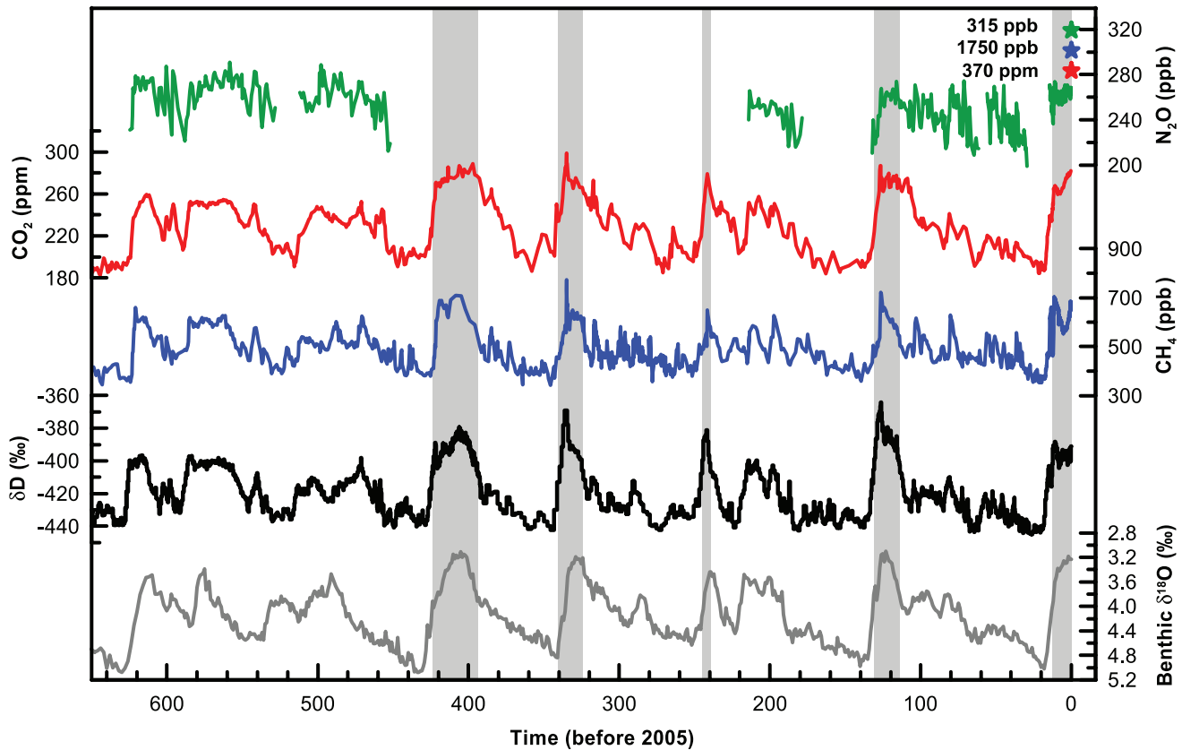
Figure 6.3. Variations of deuterium ( \delta D ; black), a proxy for local temperature, and the atmospheric concentrations of the greenhouse gases CO 2 (red), CH 4 (blue), and nitrous oxide (N 2 O; green) derived from air trapped within ice cores from Antarctica and from recent atmospheric measurements (Petit et al., 1999; Indermühle et al., 2000; EPICA community members, 2004; Spahni et al., 2005; Siegenthaler et al., 2005a,b). The shading indicates the last interglacial warm periods. Interglacial periods also existed prior to 450 ka, but these were apparently colder than the typical interglacials of the latest Quaternary. The length of the current interglacial is not unusual in the context of the last 650 kyr. The stack of 57 globally distributed benthic \delta^{18}O marine records (dark grey), a proxy for global ice volume fluctuations (Lisiecki and Raymo, 2005), is displayed for comparison with the ice core data. Downward trends in the benthic \delta^{18}O curve reflect increasing ice volumes on land. Note that the shaded vertical bars are based on the ice core age model (EPICA community members, 2004), and that the marine record is plotted on its original time scale based on tuning to the orbital parameters (Lisiecki and Raymo, 2005). The stars and labels indicate atmospheric concentrations at year 2000.
