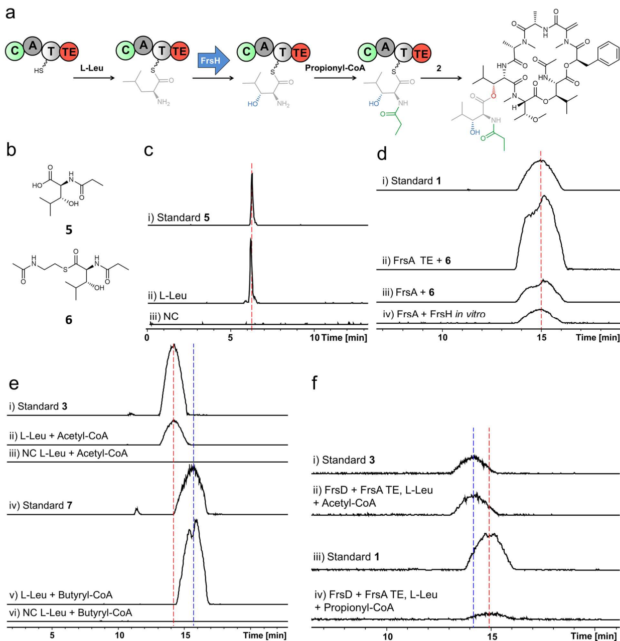
Figure 3: In vitro assays with FrsA/B, FrsH and FrsA TE . a. Reaction scheme of N -Pp-Hle formation and intermolecular transesterification onto 2 to yield 1 . b. Structures of synthesized N -Pp-Hle ( 5 ) and its SNAC ( 6 ). c. In vitro production of 5 ( m/z : 202.108). i) Synthetic 5 (1 \mu\text{g/ml} ). ii) Enzymatic assay with purified FrsA CAT /FrsB, FrsH, incubated with L-Leu and propionyl-CoA, hydrolyzed with KOH. iii) Negative control (NC) with heat inactivated protein. d. In vitro production of 1 ( m/z : 1002.540). i) 1 (10 \mu\text{g/ml} ). ii) Purified FrsA TE incubated with 6 and 2 . iii) Purified FrsA/B incubated with 6 and 2 . iv) Purified FrsA/B, FrsH incubated with propionyl-CoA, L-Leu and 2 . e. In vitro production of FR congeners 3 ( m/z : 988.530) and 7 ( m/z : 1016.550). i) 3 (10 \mu\text{g/ml} ). ii) Purified FrsA/B, FrsH incubated with L-Leu, acetyl-CoA and 2 . iii) Negative control. iv) 7 (10 \mu\text{g/ml} ). v) Purified FrsA/B, FrsH incubated with L-Leu, butyryl-CoA and 2 . vi) Negative control. f. In vitro FrsA/D combinations: i) 3 (1 \mu\text{g/ml} ). ii) Production of 3 by FrsA TE and FrsD, incubated with acetyl-CoA, L-Leu and 2 . iii) 1 (1 \mu\text{g/ml} ). iv) Production of 1 by FrsA TE and FrsD, incubated with propionyl-CoA, L-Leu and 2 .
