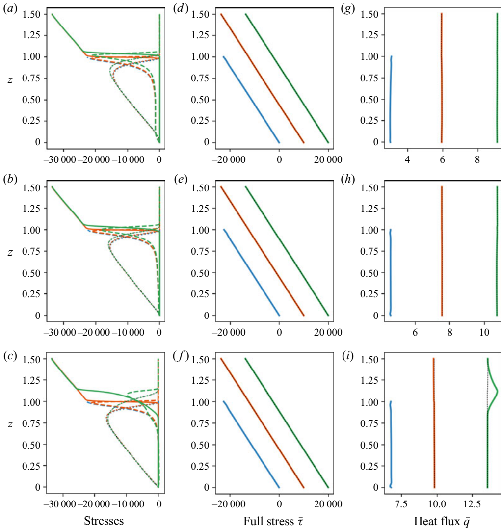
Figure 15. (a–c) Reynolds stress \tau_w (dotted lines), viscous stress \tau_v (dashed lines), linear damping stress \tau_d (solid lines) and Reynolds stress plus anomalous stress \tau_w + \bar{\tau} (for stages II and III; black dashed lines) averaged in time over 20 friction time units and horizontal planes as functions of depth z for stable, neutral and unstable stratification, respectively (see the text for more details). Blue, orange and green colours denote results obtained in stages I, II and III, respectively (same in (d–f) and (g–i)). (d–f) Total stress, i.e. \tau_w + \tau_v + \tau_d (solid lines), and total stress plus the anomalous stress, i.e. \tau_w + \tau_v + \tau_d + \bar{\tau} (thin black dashed lines), averaged in time over 20 friction time units and horizontal planes as functions of depth z for stable, neutral and unstable stratification, respectively. Note that the full stress is shifted to the right by 10 000 (20 000) between stage II and stage I and between stage III and stage II for the case of stable (unstable) stratification for clarity as all curves overlap otherwise. (g–i) Heat flux q (solid lines) and heat flux plus anomalous heat flux q + \bar{q} (thin black dashed lines) averaged in time over 20 friction time units and horizontal planes as functions of depth z for stable, neutral and unstable stratification, respectively. Note that the heat flux is shifted to the right by 2.5 (5) between stage II and stage I and between stage III and stage II for the case of stable (unstable) stratification for clarity.
