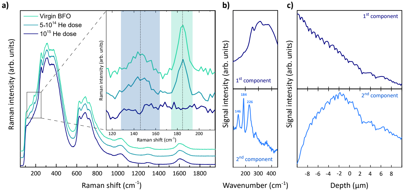
FIG. 2: (a) Raman spectra performed on different regions of the \text{BiFeO}_3//\text{SrTiO}_3 film. The underlying intense signal of \text{SrTiO}_3 is very visible but some \text{BiFeO}_3 phonon modes can be singled out. The inset shows these phonon modes, with a baseline subtraction. The colored regions and dotted lines are guides for the viewer. (b,c) Principal component analysis of the depth profiles on a non-implanted region of the film: we can see the component signal (b) and the associated depth profiles (c) for the first two components.
