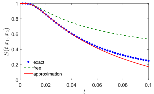
FIG. 2: Time evolution of the survival probability as given by the exact solution (13), the free solution (5) and Eq. (23). The chosen parameter values are x_1 = 0.9 , x_2 = 0.1 , D_1 = 1 , and D_2 = 5 , leading to r_0 \approx 0.901 , \Theta \approx 0.421 , and \theta_0 \approx 0.05 .
