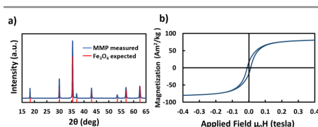
Fig. 2 (a) X ray diffraction spectra and (b) magnetization curve of MMP obtained after 4 h of ball milling.
