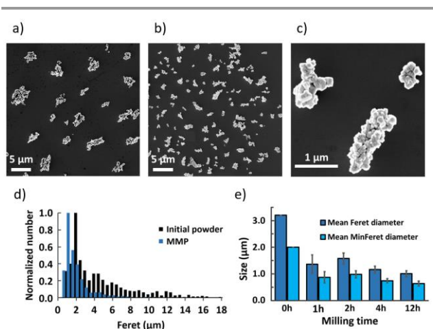
Fig. 1 SEM images of the initial powder (a) and particles after 4 h of ball milling (b, c). (d) Feret diameter distribution for the initial powder and for particles after 4 h of ball milling (MMP). (e) Mean Feret and Mean MinFerret diameters for the initial powder and after 1, 2, 4 and 12 h of ball milling, calculated from the lognormal size distribution fitting.
