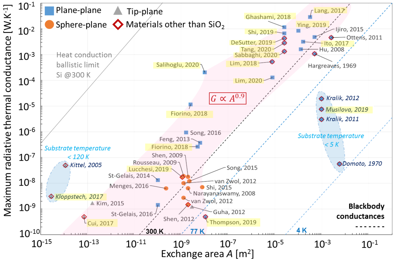
Fig. 3: Analysis of the maximal thermal conductance in near-field thermal radiation experiments as a function of exchange area. Blackbody conductances (dashed lines) are provided as references, as well as the maximal (ballistic) thermal conductance associated with heat conduction inside a solid (Si).
