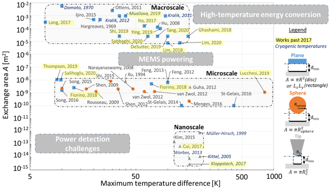
Fig. 2: Classification of the experiments involving near-field radiative heat transfer according to exchange area and temperature difference.
