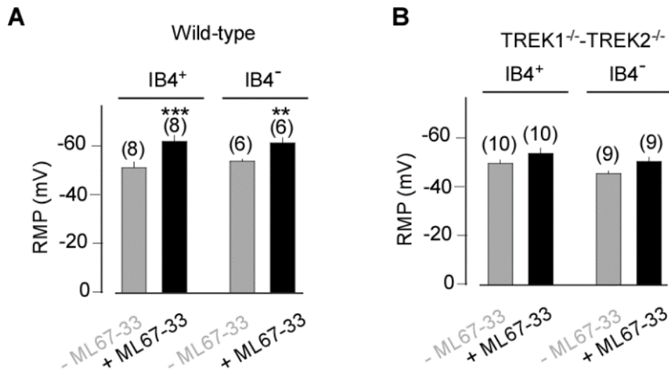
1 2 3 Figure S3. ML67-33 hyperpolarizes TG neurons from wild-type mice through activation 4 of TREK channels, Related to Figure 3. (A-B) Bar graphs showing representing the RMP 5 value obtained from small IB4 + and IB4 - TG neurons before and after perfusion with ML67-33 6 (10 \mu M) from wild-type (A) and Trek1 -/- - Trek2 -/- (B) mice. Paired t-test (** p < 0.01, *** p < 7 0.001). Mean \pm SEM.
