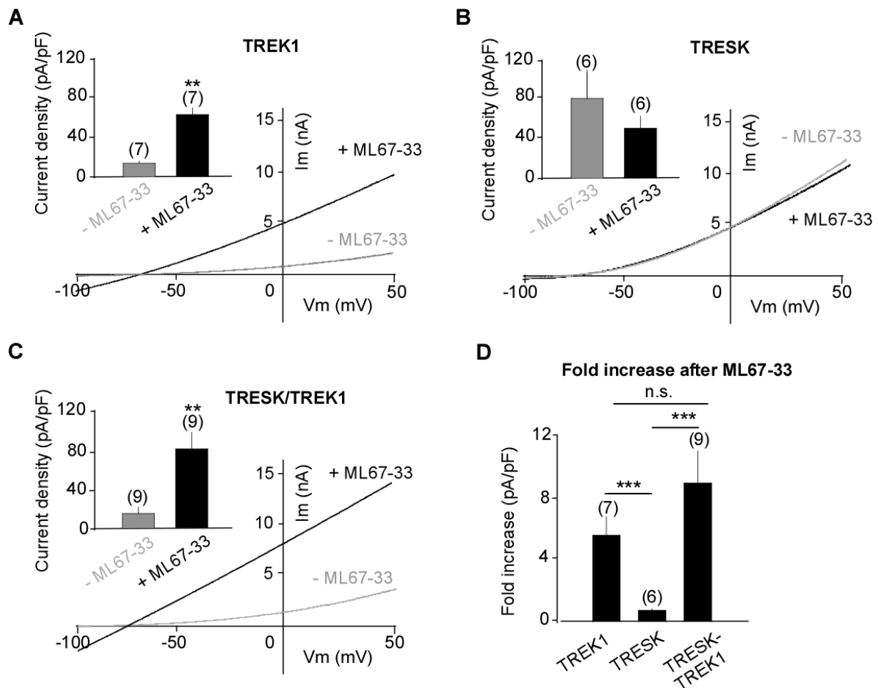
3 Figure S1. ML67-33 activates TREK1 homodimers and TRESK/TREK1 heterodimers 4 but not TRESK homodimers, Related to Figure 2 and 3. (A-C) Representative current traces 5 obtained from HEK293T cells expressing either TREK1 (A) or TRESK (B) homodimers or 6 TRESK/TREK1 (C) heterodimers before and after application of ML67-33 (10 \mu M). Currents 7 were elicited by voltage-ramps (from -100 to +100 mV from a holding potential at -80 mV, 1s 8 duration). Insets show a summary of current densities obtained at 0 mV. Paired t-test (** p < 9 0.01). (D) Bar graph showing the fold increase after perfusion with ML67-33. Kruskal-Wallis 10 and Student-Newman-Keuls post hoc (***) p < 0.001). Mean \pm SEM.
