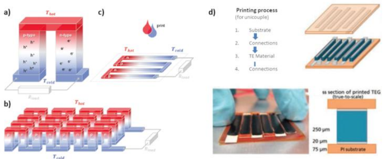
Figure 3: Schematics of (a) a thermoelectric element, which comprises one n - and one p -type thermoelectric leg that experience a temperature gradient \Delta T = T_{hot} - T_{cold} leading to charge accumulation at the cold ends, (b) a conventional thermoelectric module that comprises an array of elements, which are connected electrically in series but thermally in parallel, and (c) an in-plane (printable) array of elements. generators (according to ref. 77 reproduced with permission from the Royal Society of Chemistry). From the perspective of applications, thermoelectric generators (TEGs) containing a large number of thermoelectric p - and n -type legs connected in series are needed to achieve considerable power output. Bulk PCPs are compatible with vertical device geometry. d) From the perspective of evaluating the performances of a material, connecting in series vertical mono leg TEG (only one type of polymer) can be easily produced. In this case, a conductive electrode (gold or silver paste) is replacing the second type of leg. The printing sequence, scheme of a
