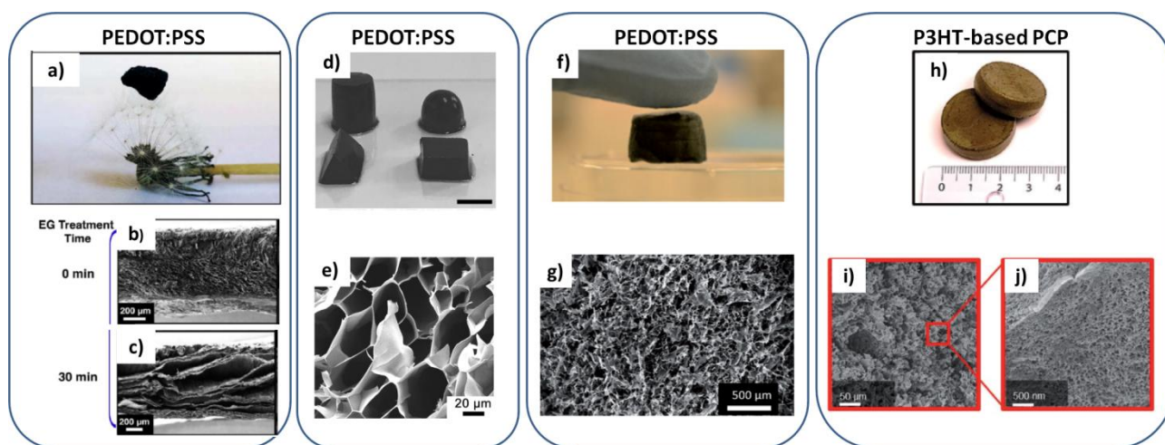
Figure 5 : Different PCP states and their macroporous structure observed by SEM. a - c) ultra-low density PEDOT:PSS cryogel placed on top of a dandelion and SEM characterizations of the gel before and after treatment with EG; 21 d - e) Digital pictures of PEDOT:PSS hydrogels with different geometric shapes (scale bars = 1 cm) and cross-section SEM image of a freeze-dried PEDOT:PSS hydrogel and after the treatment with concentrated H_2SO_4 ; 10 f - g) PEDOT:PSS, GOPS, and NFC PCP composite and SEM image of the internal structure; 25 h - j) P3HT “foam” and its internal porous structure characterized by SEM. 28 All panels have been reproduced with permission from J. APPL. POLYM. SCI. (a-c), Adv. Mater. (d-e), Adv. Funct. Mater. (f-g and h-j).
