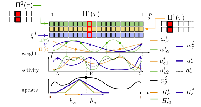
Fig. 2. Weights, activity, and neighborhood functions in a map being connected to two other maps in CxSOM. The external activity has three maxima A, B, and C. The global activity corresponds to the external one modulated by the contextual activity. It allows the map to select the best matching unit at a position close to B, as both the contextual activities are high only in this area.
