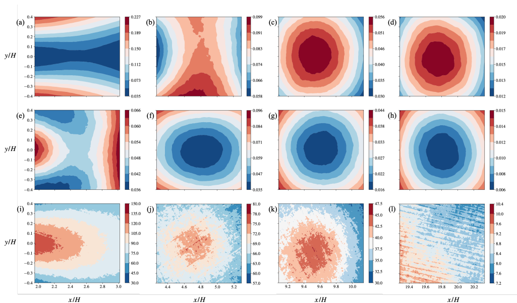
Figure 15: Isocontours of (a - d) coherent turbulent kinetic energy \overline{k}/U_\infty^2 , (e - h) remaining small-scale turbulent kinetic energy \overline{k'}/U_\infty^2 , and (i - l) energy dissipation rate \overline{\epsilon'} in the SFVs corresponding to G/H = 2.4 at Re = 1.0 \times 10^4 . (a, e, i): SFV2.5, (b, f, j): SFV5, (c, g, k): SFV10, and (d, h, l): SFV20.
