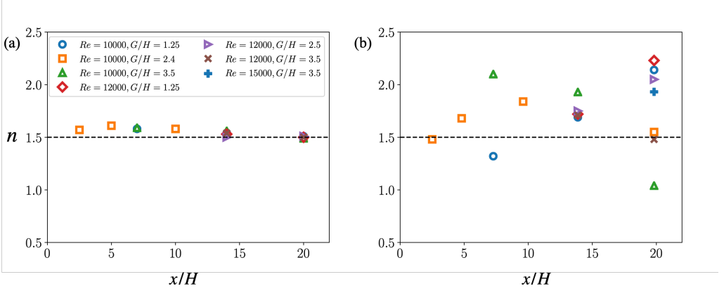
Figure 21: Scaling exponent n in (a) C'_\epsilon \sim Re'_\lambda{}^{-n} for the flow fields reconstructed based on random motions (POD modes 3 to 2000) and in (b) C_\epsilon \sim Re_\lambda{}^{-n} for the flow fields with coherent motions. The different values of x/H correspond to different SFVs.
